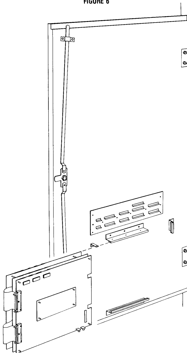
PRINTED CIRCUIT BOARD REPLACEMENT FIGURE 6
