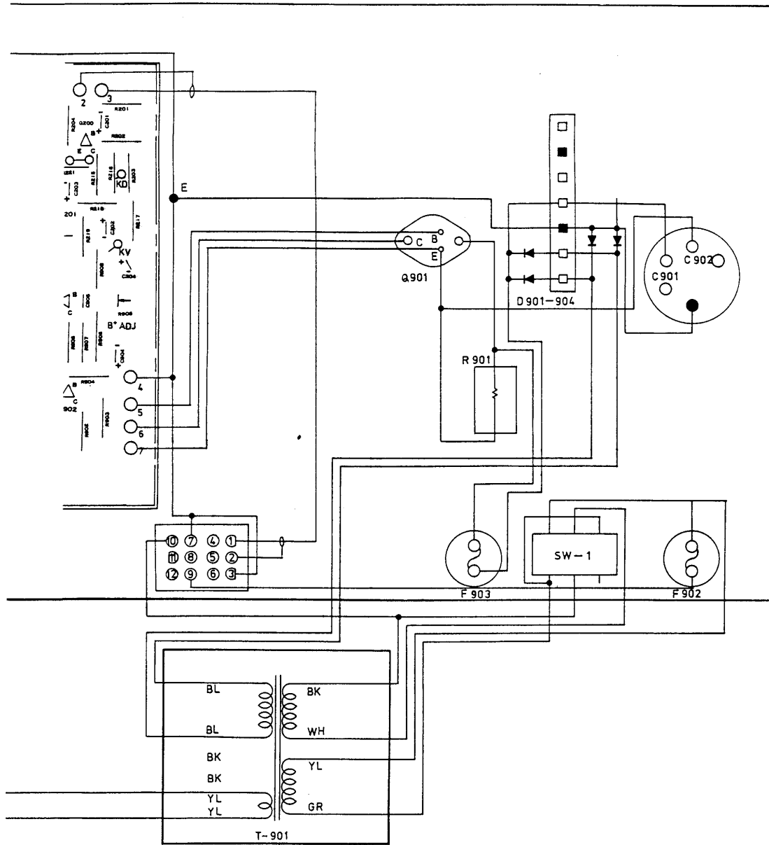
BOTTOM VIEW
