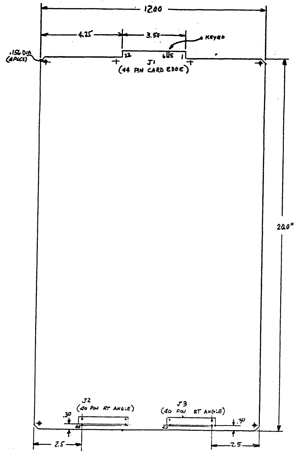
BOARD OUTLINE (NOT TO SCALE) COMPONENT SIDE SHOWN
