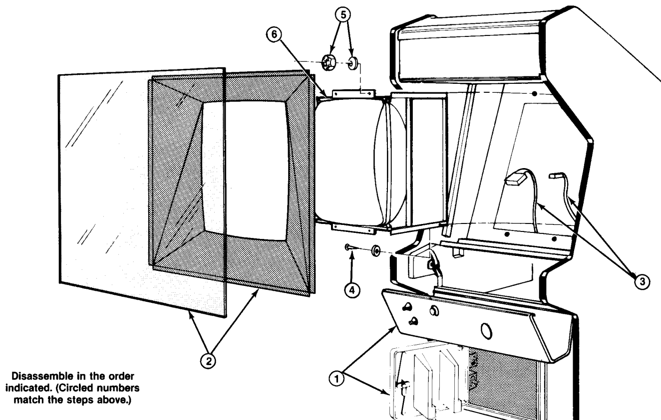
Figure 12 Monitor Removal
