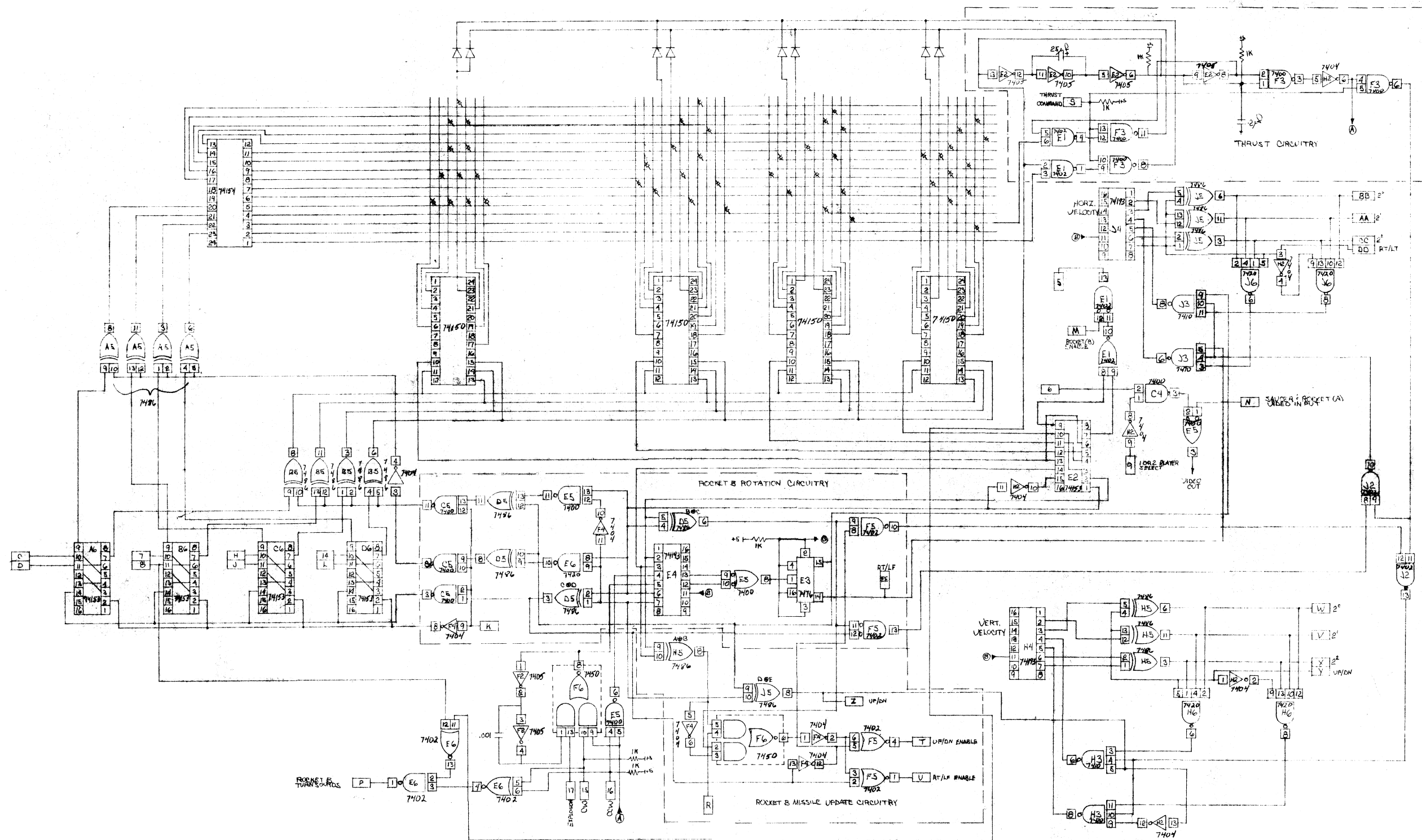
B-MEMORY 10R2 PLAYER NA 73-103 COMPUTER SPACE DRAWN BY: WALTER ANDERSON 1/29/73
