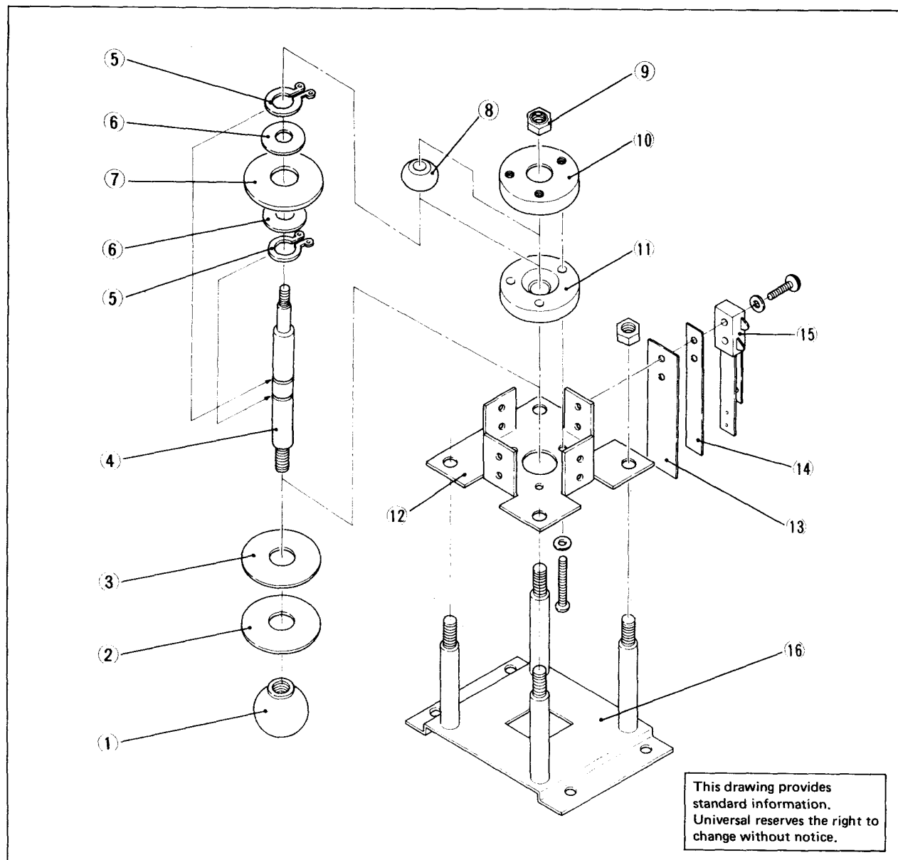
Fig. 12 Lever Assembly
