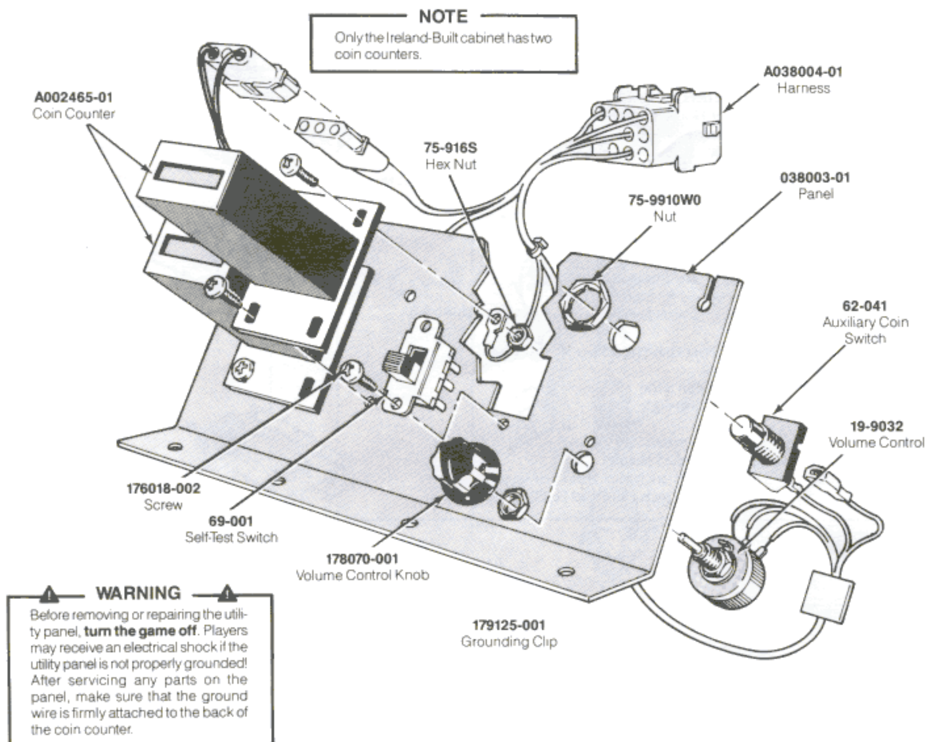
Figure 4-4 Utility Panel Assembly A038002-01 H Parts List
