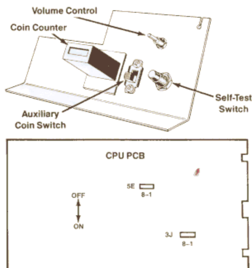
Figure 1-2 Switch Locations
