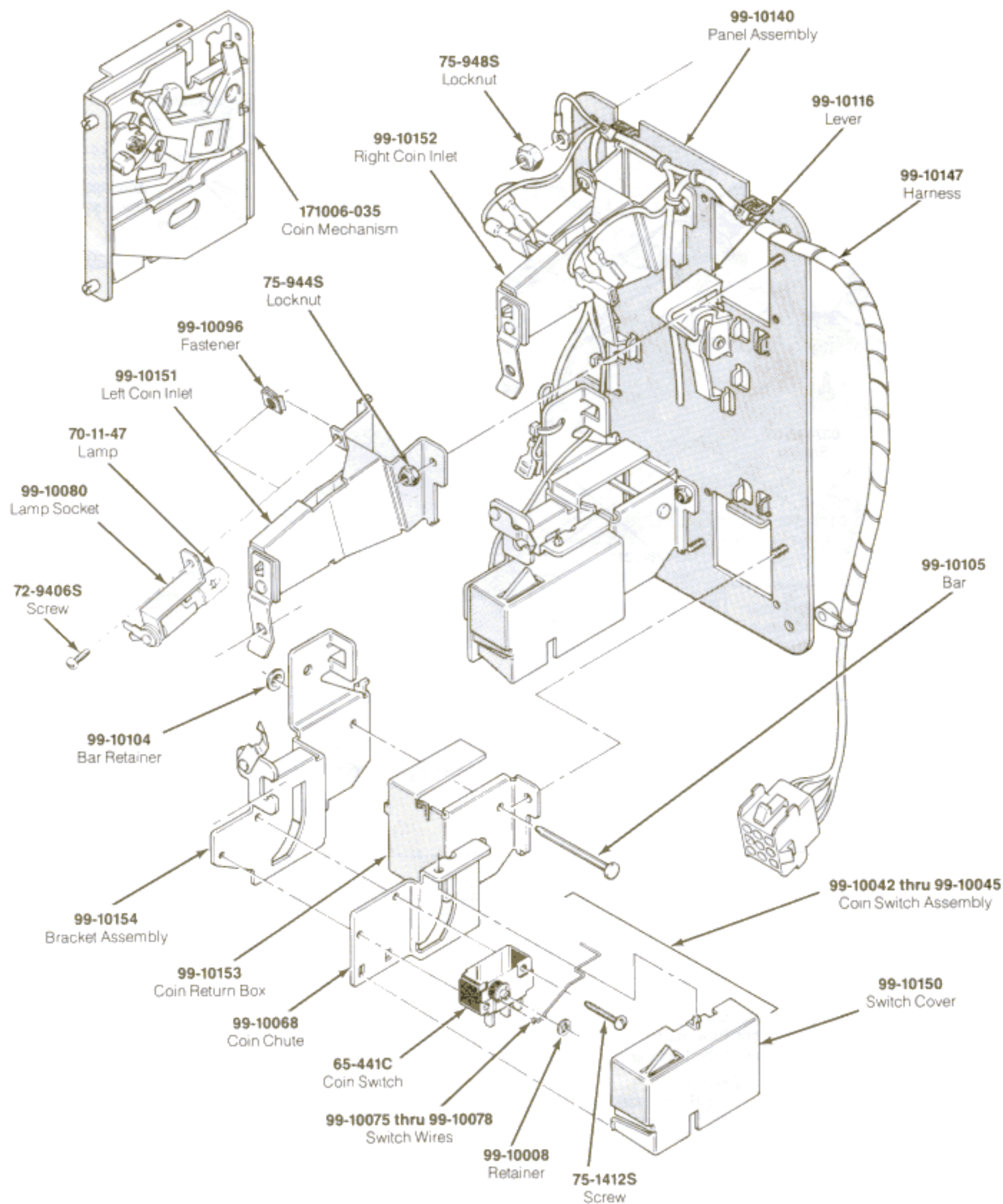
Figure 4-6 Coin Controls, Inc. Coin Door Assembly 171034-xxx A
