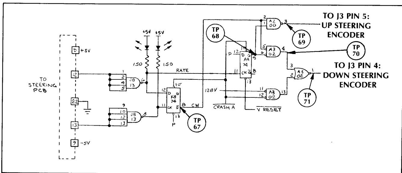
Figure 2-19 Steering Control
