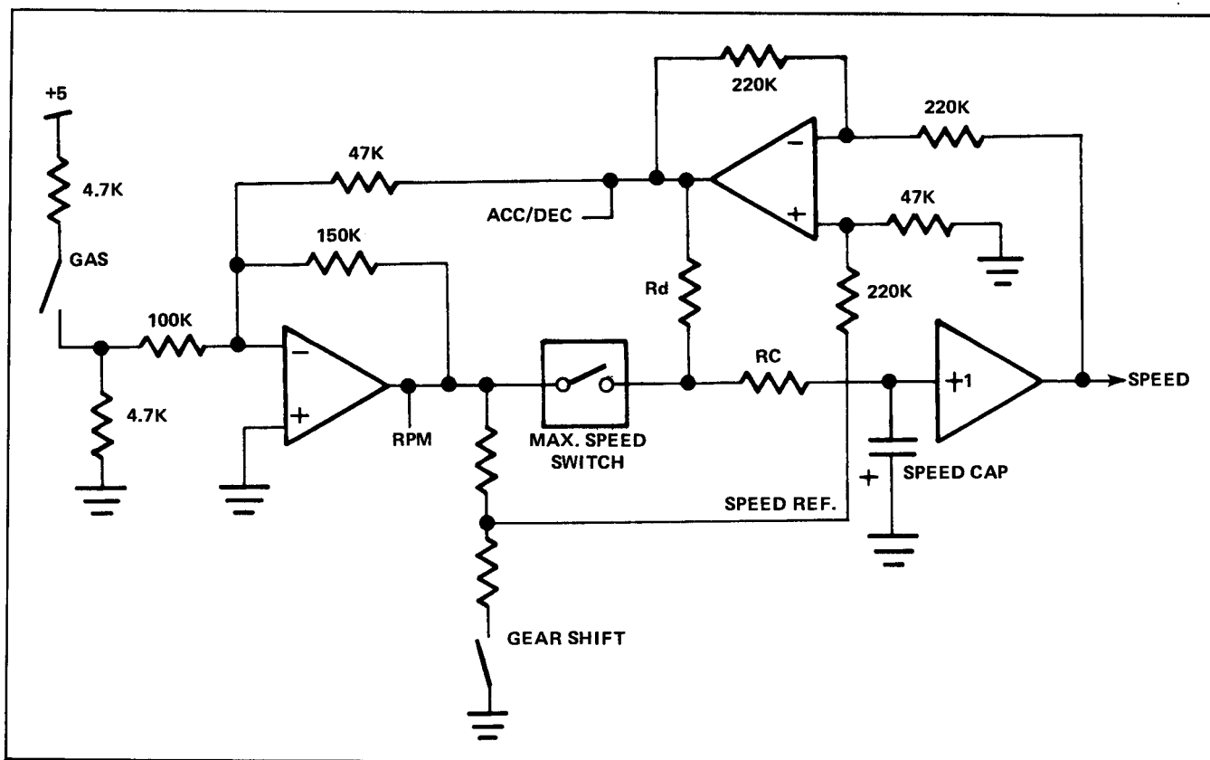
Figure 2-11 Acceleration/Deceleration Circuit
