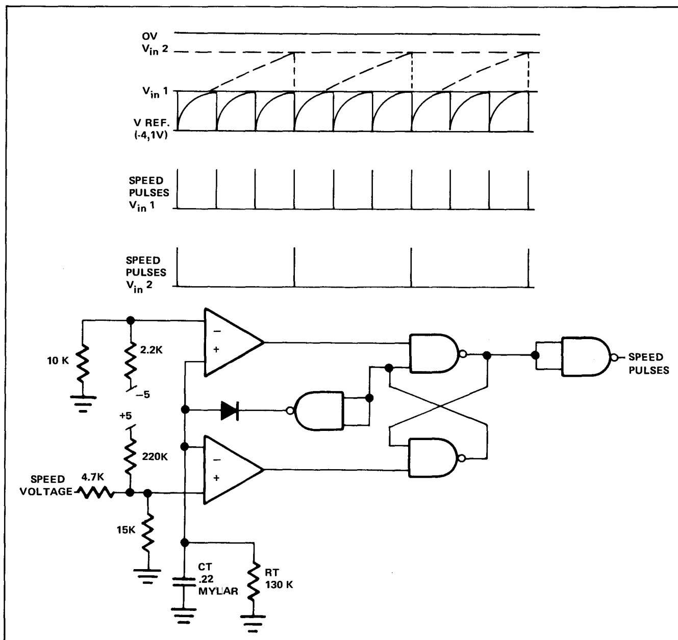
Figure 2-13 Speed Oscillator and Waveforms
