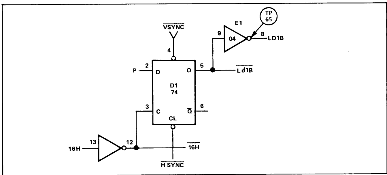
Figure 2-17 Ld1B Circuit
