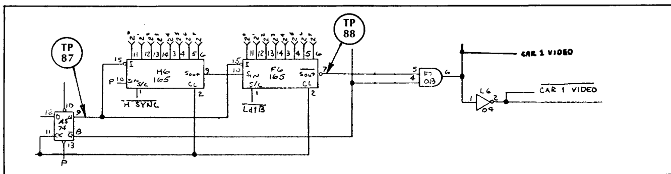
Figure 2-30 Car Display
