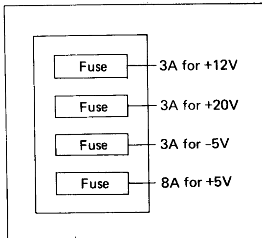
Fig. 7 Fuses in the Power Circuit Board
