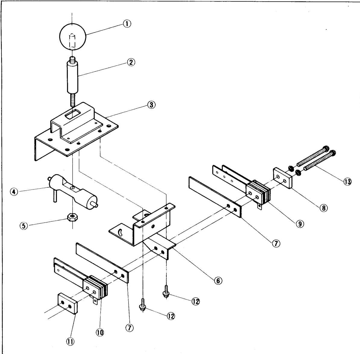
Fig. 11 Lever Assembly
