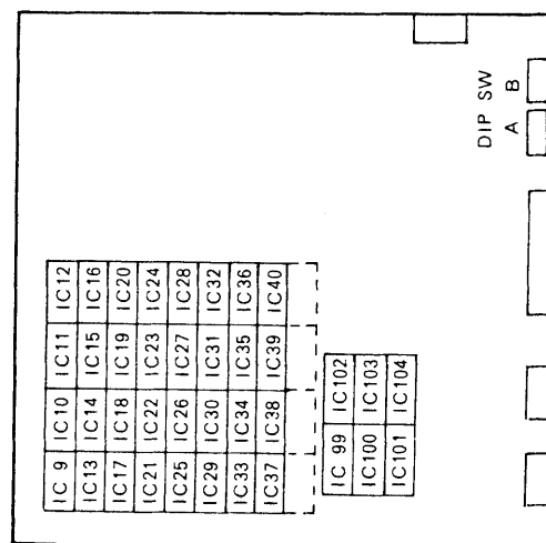
③ VIDEO BD OUT RUN 837-6064-01 (02)
