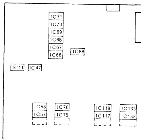
② CPU BD OUT RUN 837-6063-02
