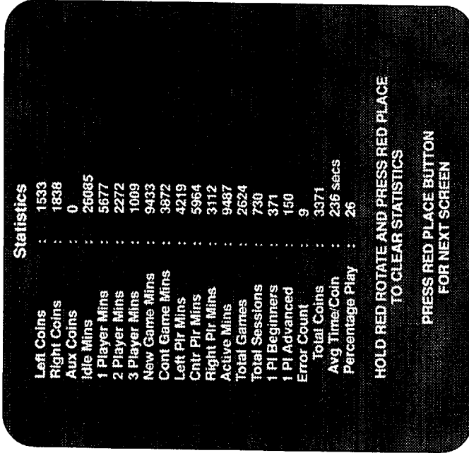
Figure 2-2 Statistics Screen
