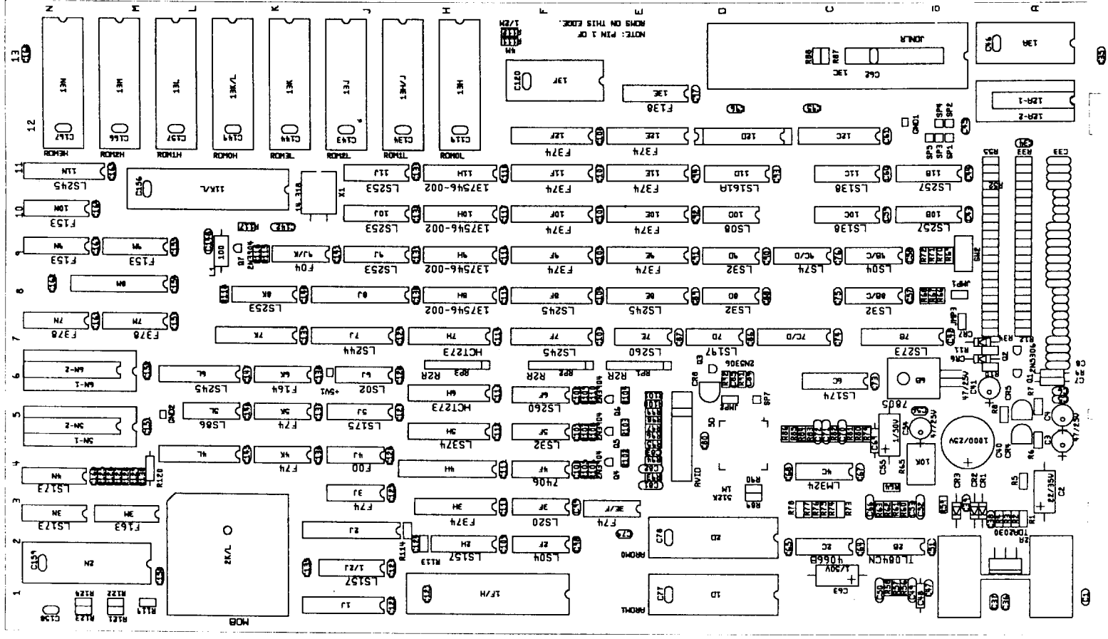
Figure 4-6 Rampart Game PCB Assembly (3-Player Version) A048868-01 D
