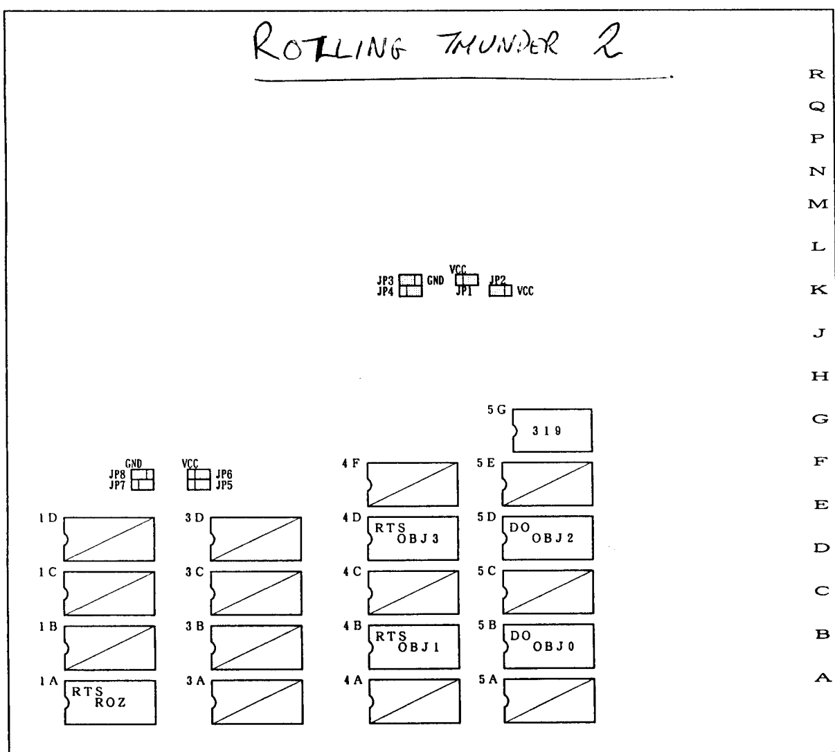
図6 (VIDEO-PCボード)
