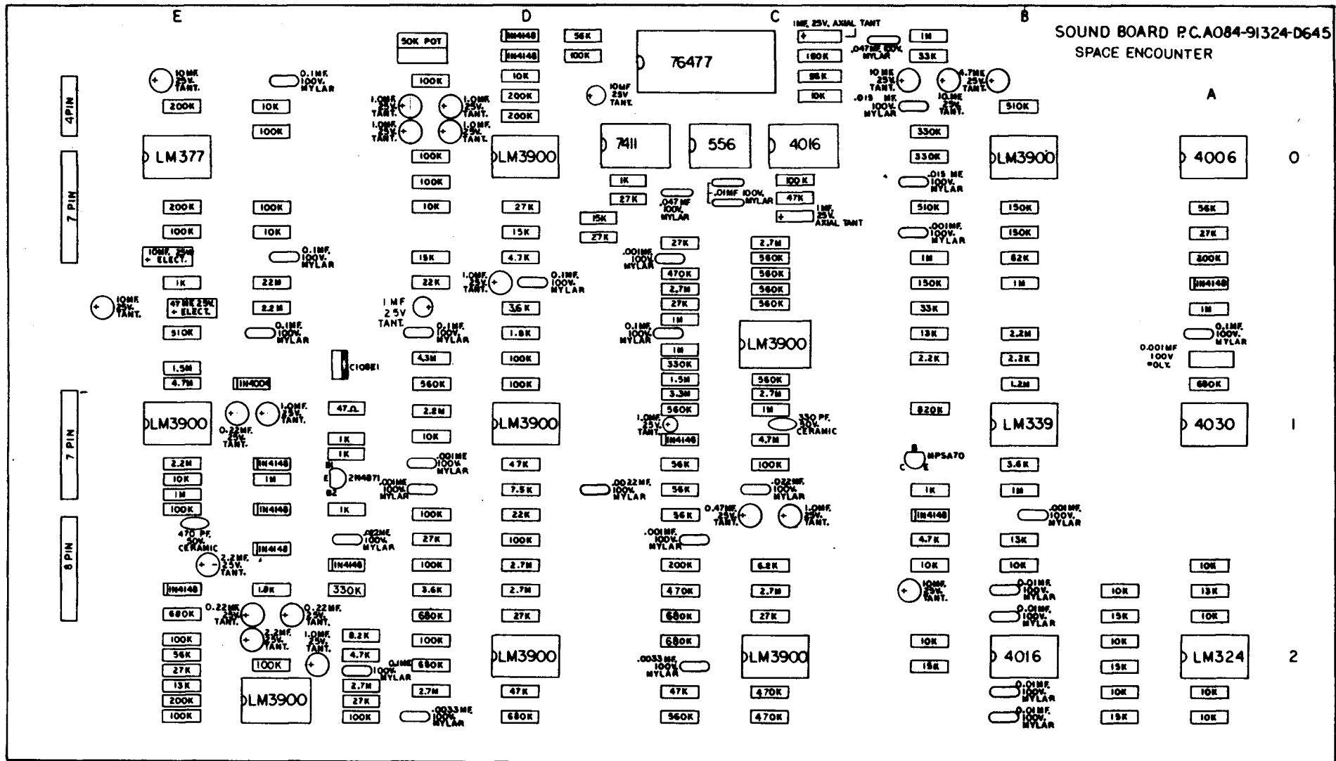
COMPONENT LAYOUT PART NO. MO51-00645-A005
