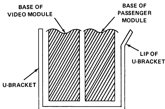
FIGURE 1. U-BRACKET PLACEMENT
