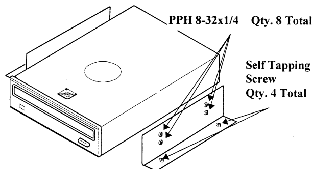
Figure 9: CD-DRIVE Mounting
