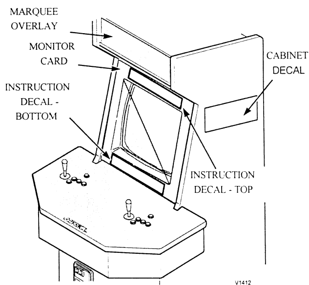
Figure 13: Cabinet Graphics
