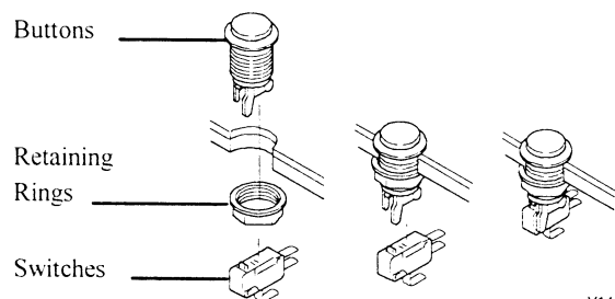
FIGURE 5 : Control Panel Buttons (“B” Kit)
