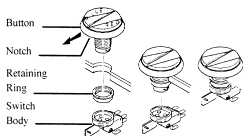
FIGURE 3 : Dual-Button Switch Installation (“Full” Kit)
