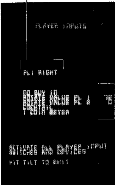
Figure 3-2b Self-Test—Player Input
