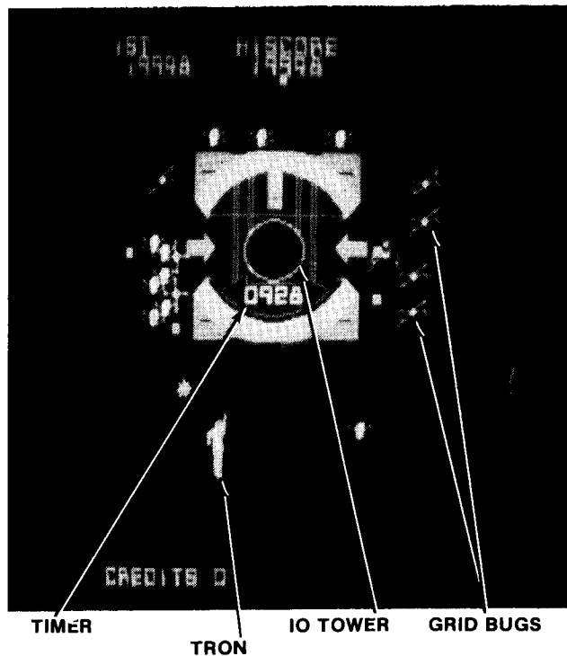
Figure 3-1 Game Operation
