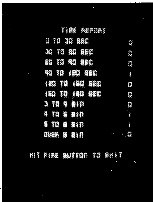
Figure 3-2d Self-Test—Time Report
