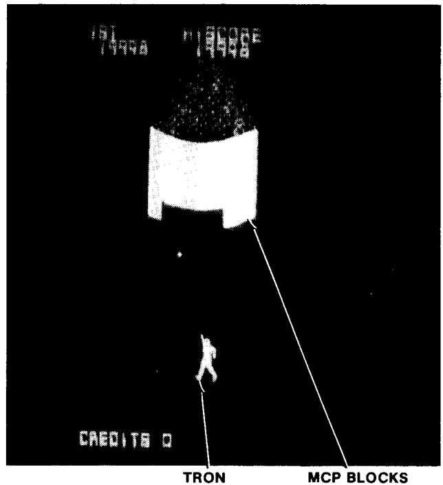
Figure 3-1 Game Operation
