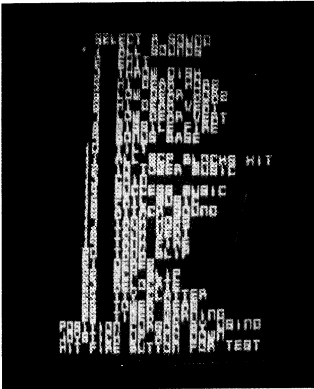
Figure 3-2a Self-Test—Sounds
