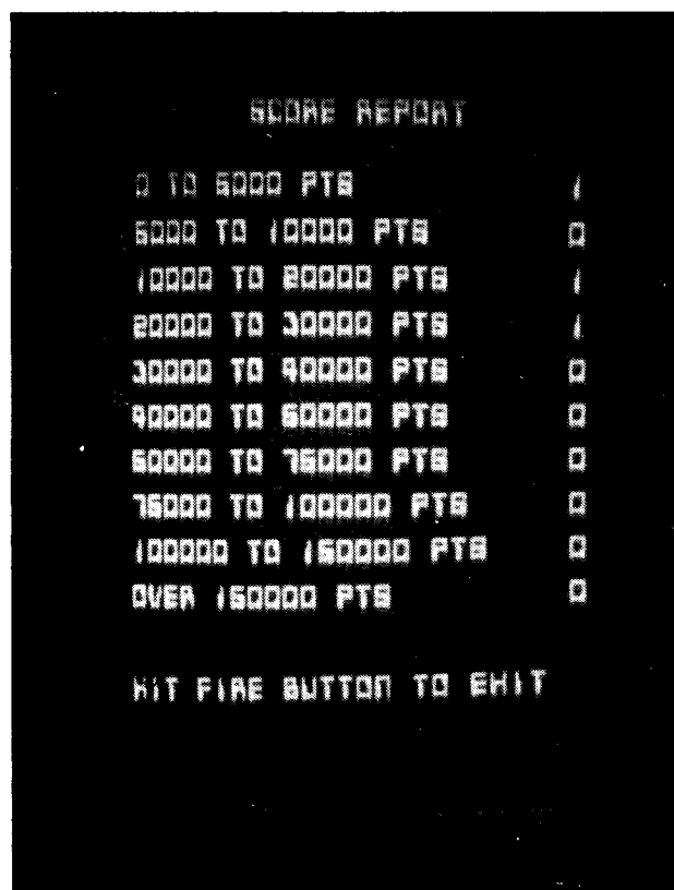
Figure 3-2e Self-Test—Score Report
