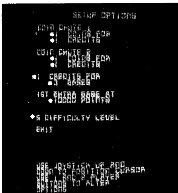
Figure 3-2f Self-Test—Setup Options
