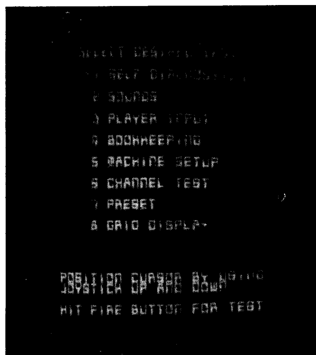
Figure 3-2 Self-Test—Menu
