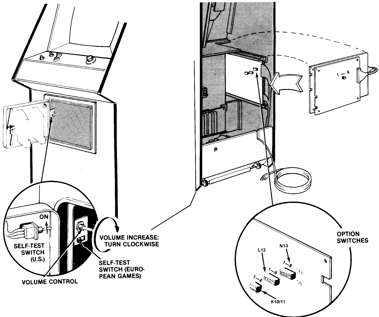
Figure 5 Location of Self-Test Switch, Volume Control and Option Switches
