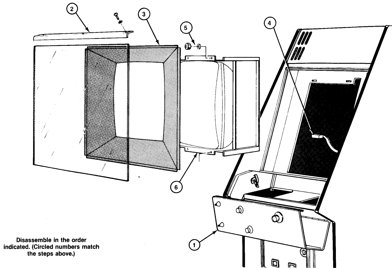
Figure 13 Monitor Removal
