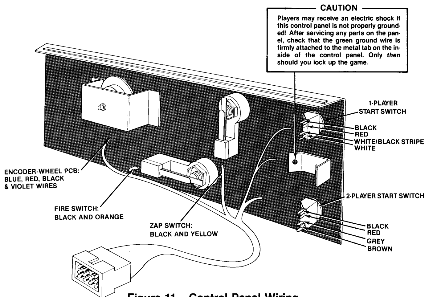
Figure 11 Control Panel Wiring
