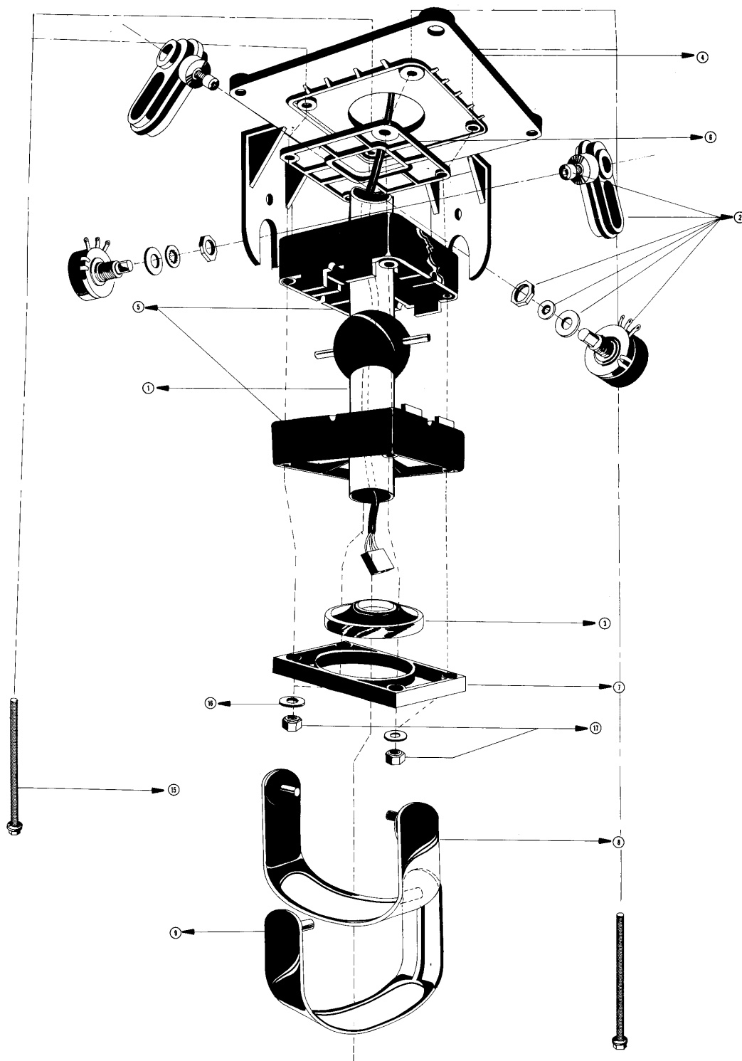
JOY STICK(UNDERSIDE)ASS'Y.
