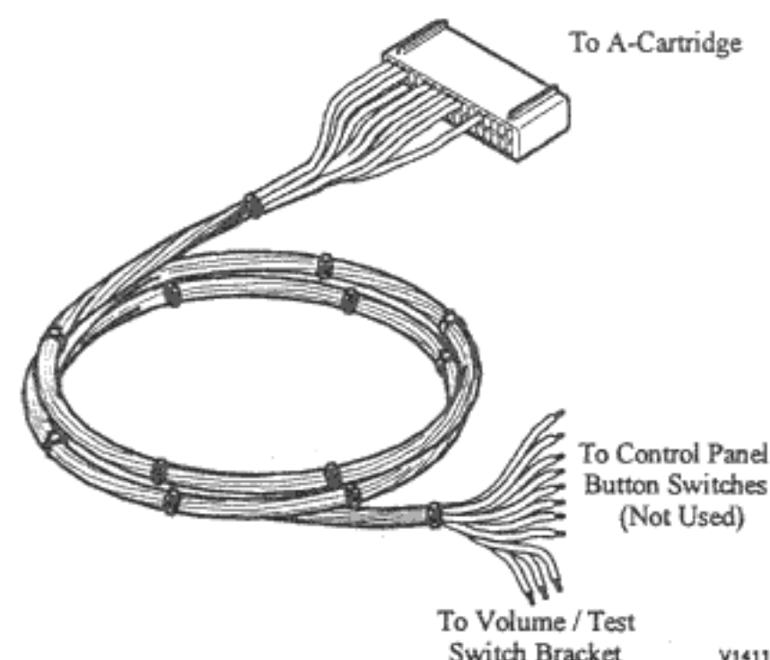
Figure 6: Auxiliary Cable Harness
