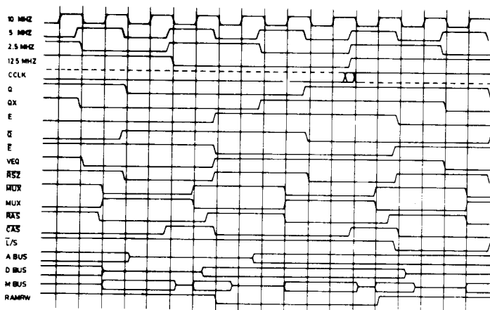
FIGURE 3-1 CLOCK TIMING
