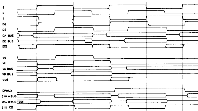
FIGURE 3-2 DUAL PORT RAM TIMING
