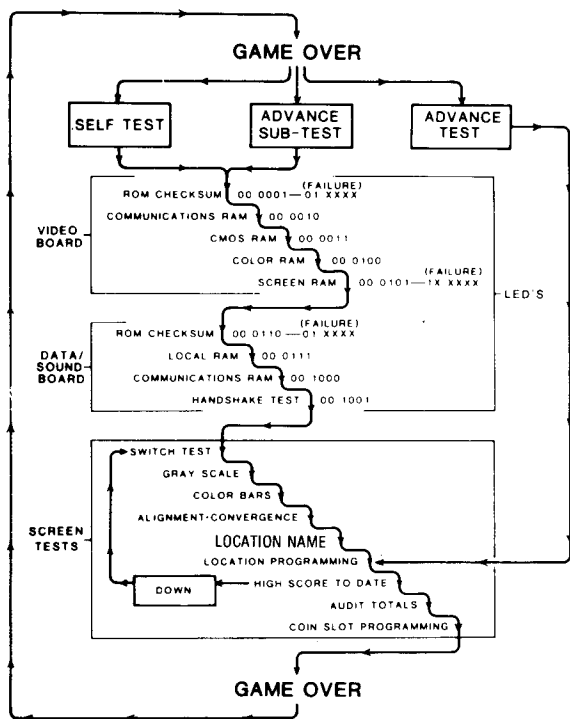
FIGURE 1-8 FLOW CHART
