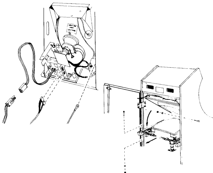
FIGURE 2-3 MONITOR REMOVAL
