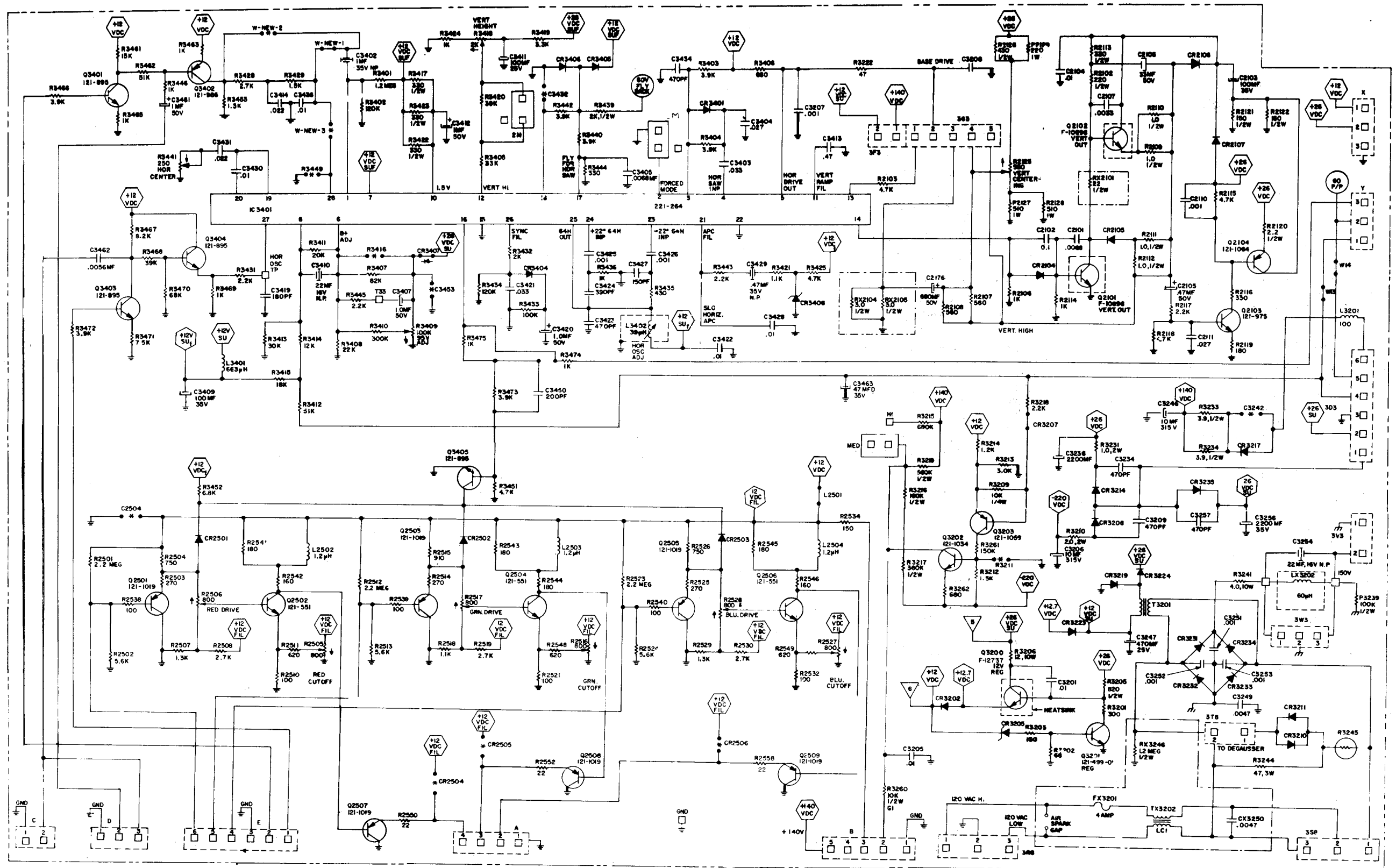
SCHEMATIC FOR 9-227-01 RGB COLOR MONITOR (MAIN BOARD) ZENITH RADIO CORP. CHICAGO, ILL. C 9-227 M051-00087-A024
