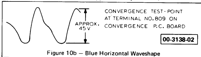
Figure 10b — Blue Horizontal Waveshape
