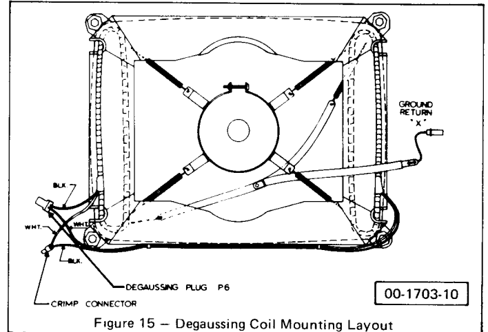
Figure 15 - Degaussing Coil Mounting Layout
