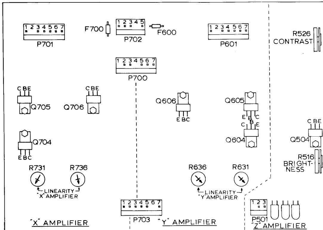
DEFLECTION AMPLIFIER PCB — Figure 3
