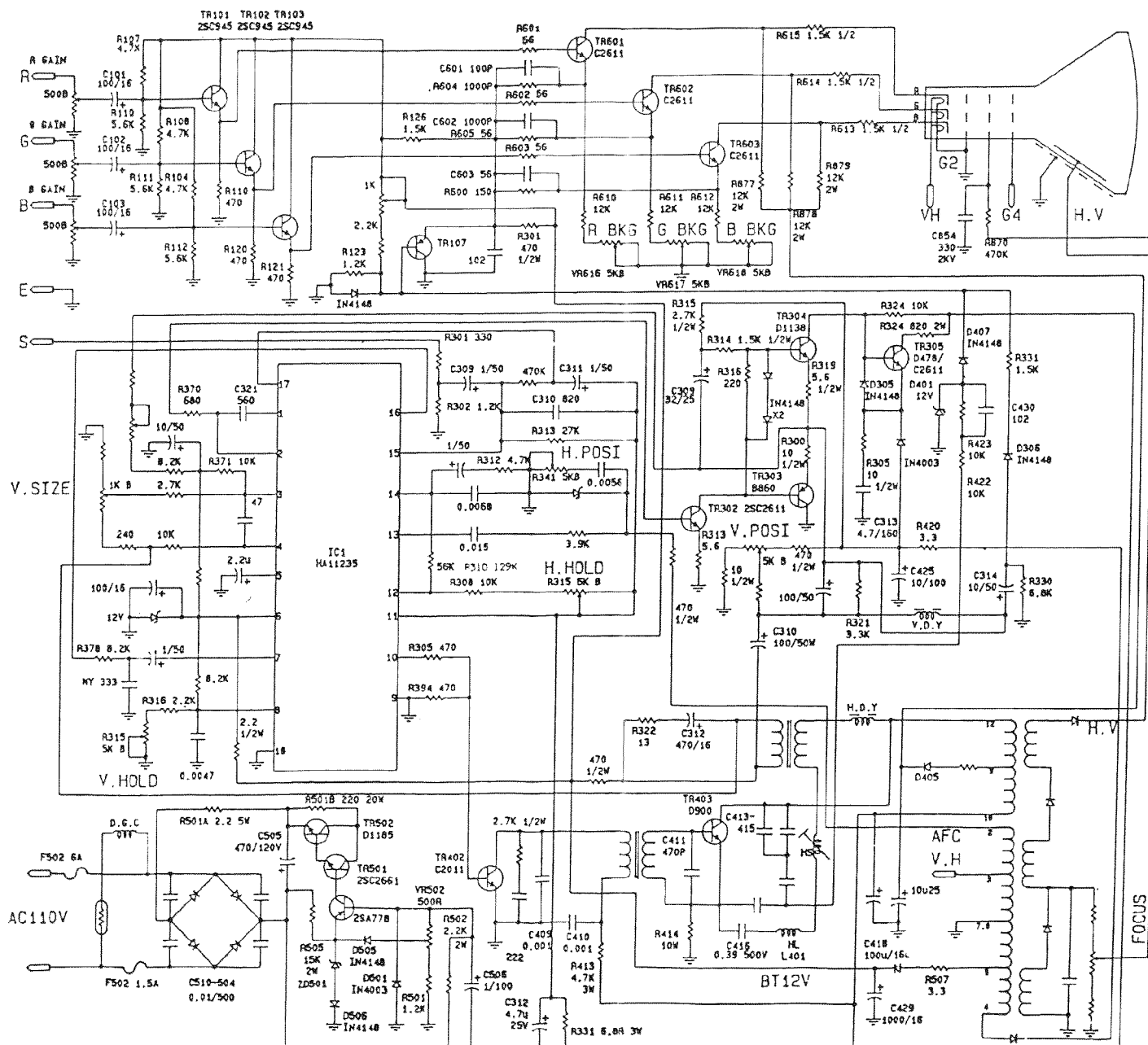
814/820/822 CHASSIS CIRCUIT DIAGRAM HUA I ELECTRONICS CO., LTD.
