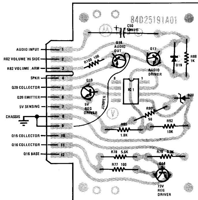
Circuit Side
