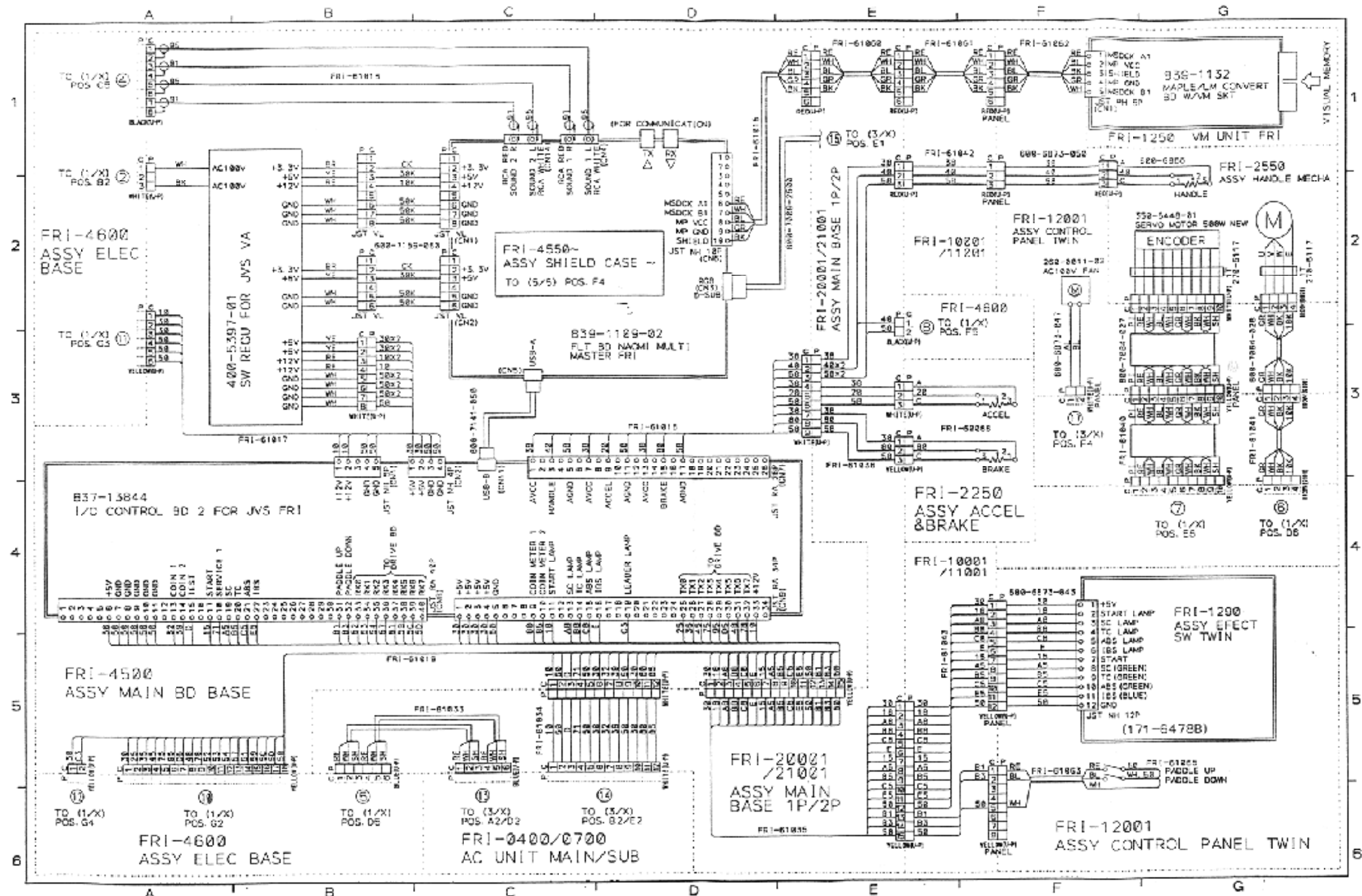
23. WIRING DIAGRAM (D-2/5)
