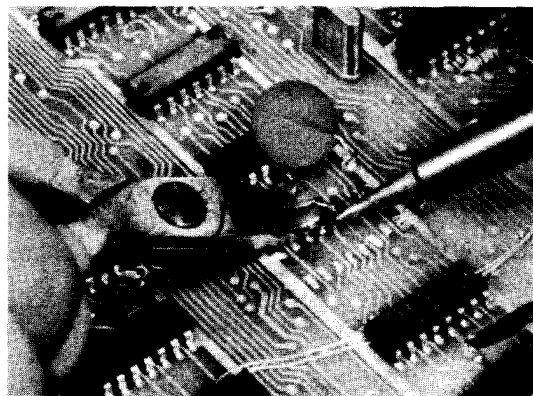
Figure 31 Removing IC Pin with Tip Dykes
