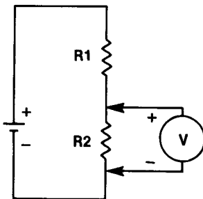
Figure 9 Schematic Diagram of Voltage Measurement Made in Figure 8
