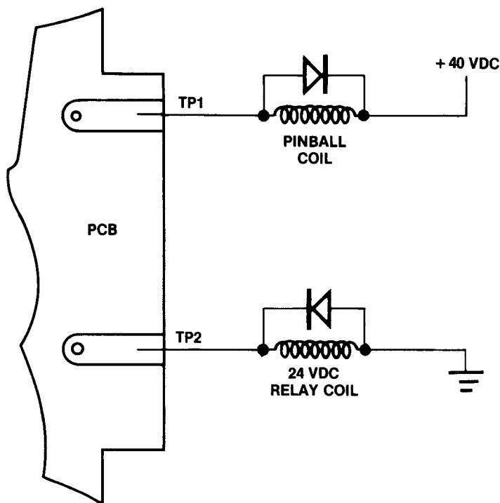
Figure 6 Troubleshooting Solenoids
