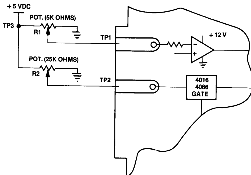
Figure 2 Troubleshooting Potentiometers
