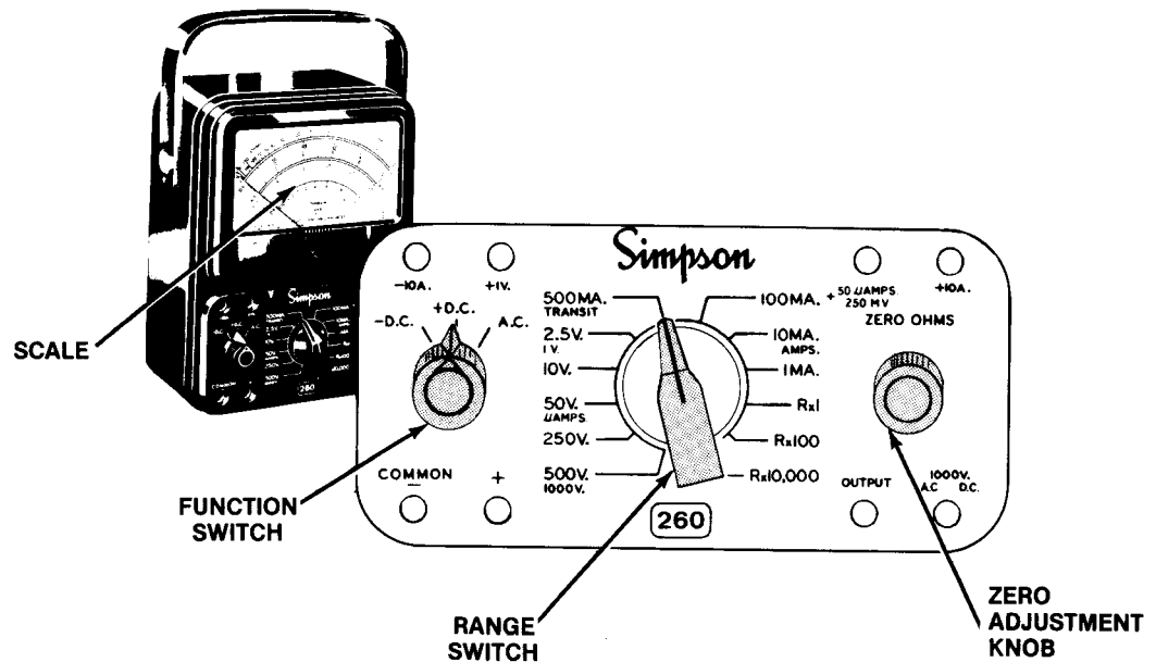
Figure 19 Simpson 260® Meter
