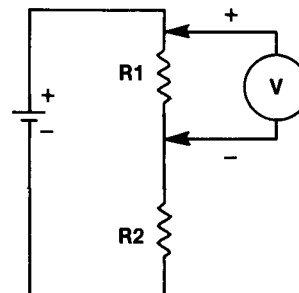
Figure 10 Schematic Diagram of Another Voltage Measurement
