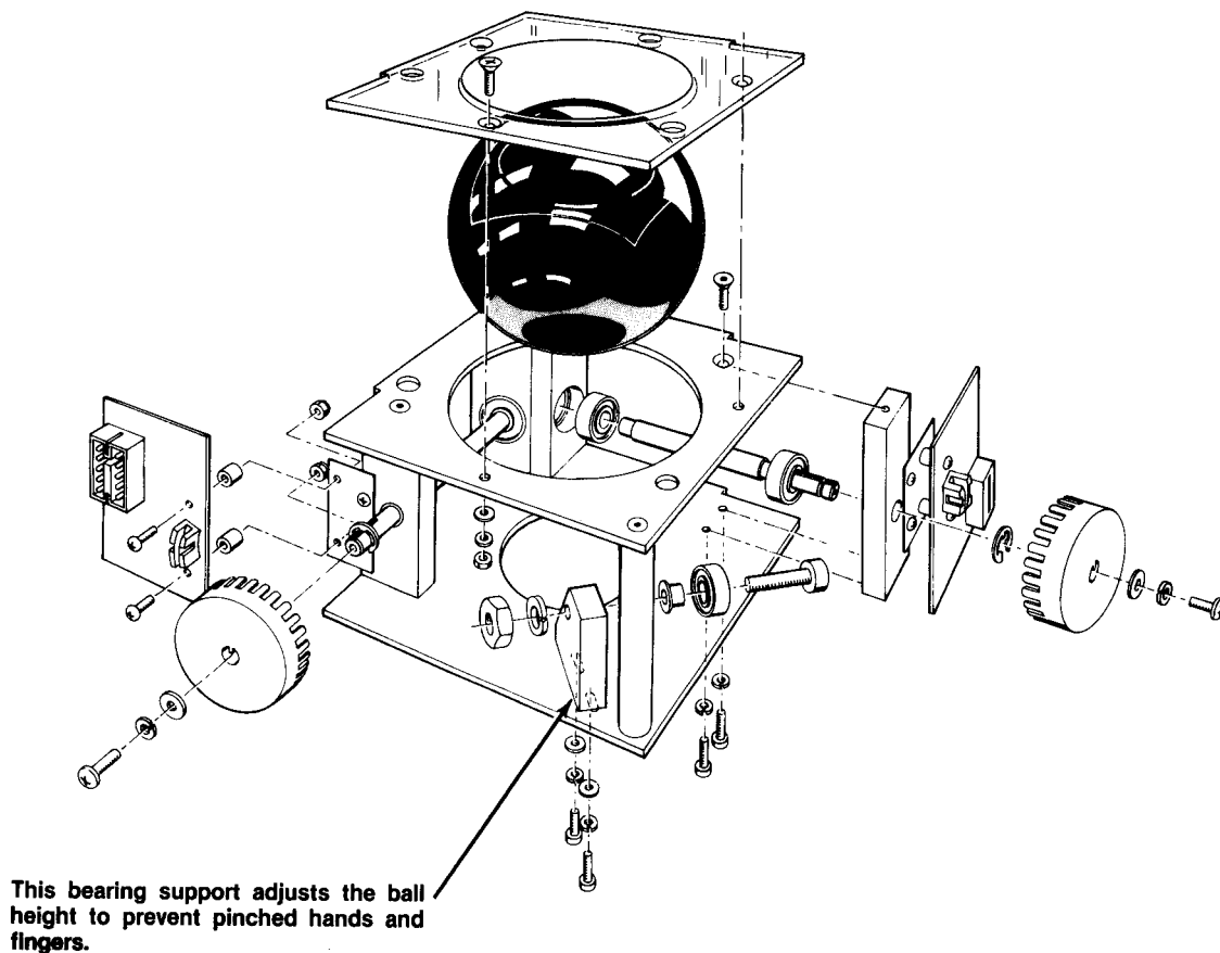
Figure 11 Trak Ball™ Assembly
