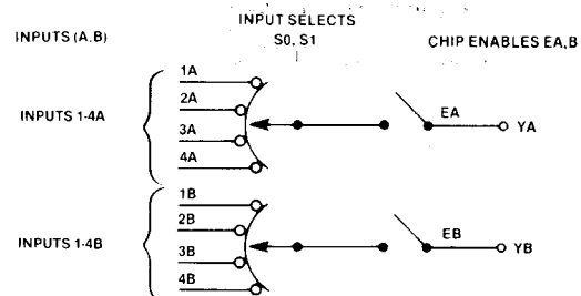
SWITCH LOGIC FOR A 74153
