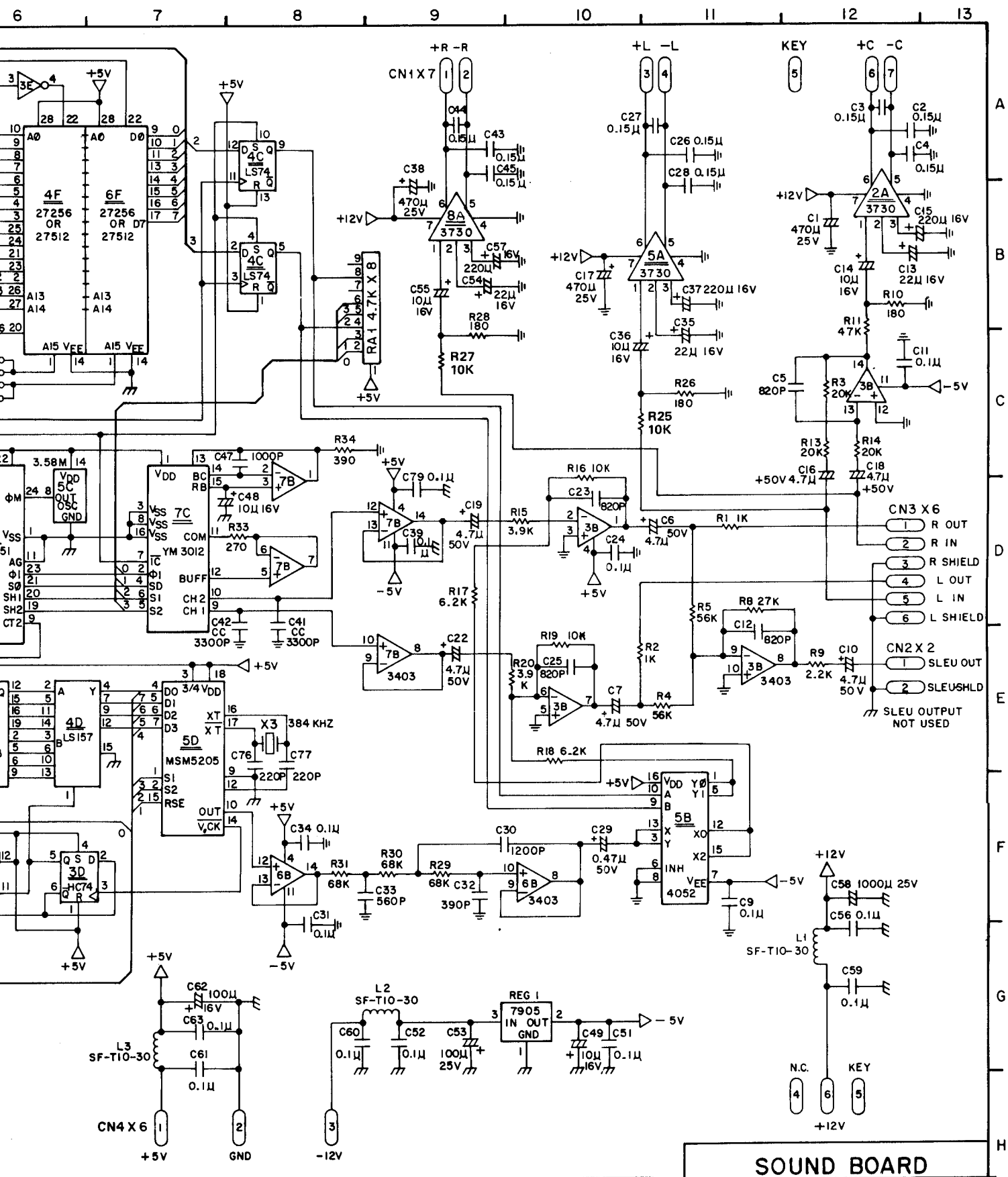
Sound Board Logic Diagram
