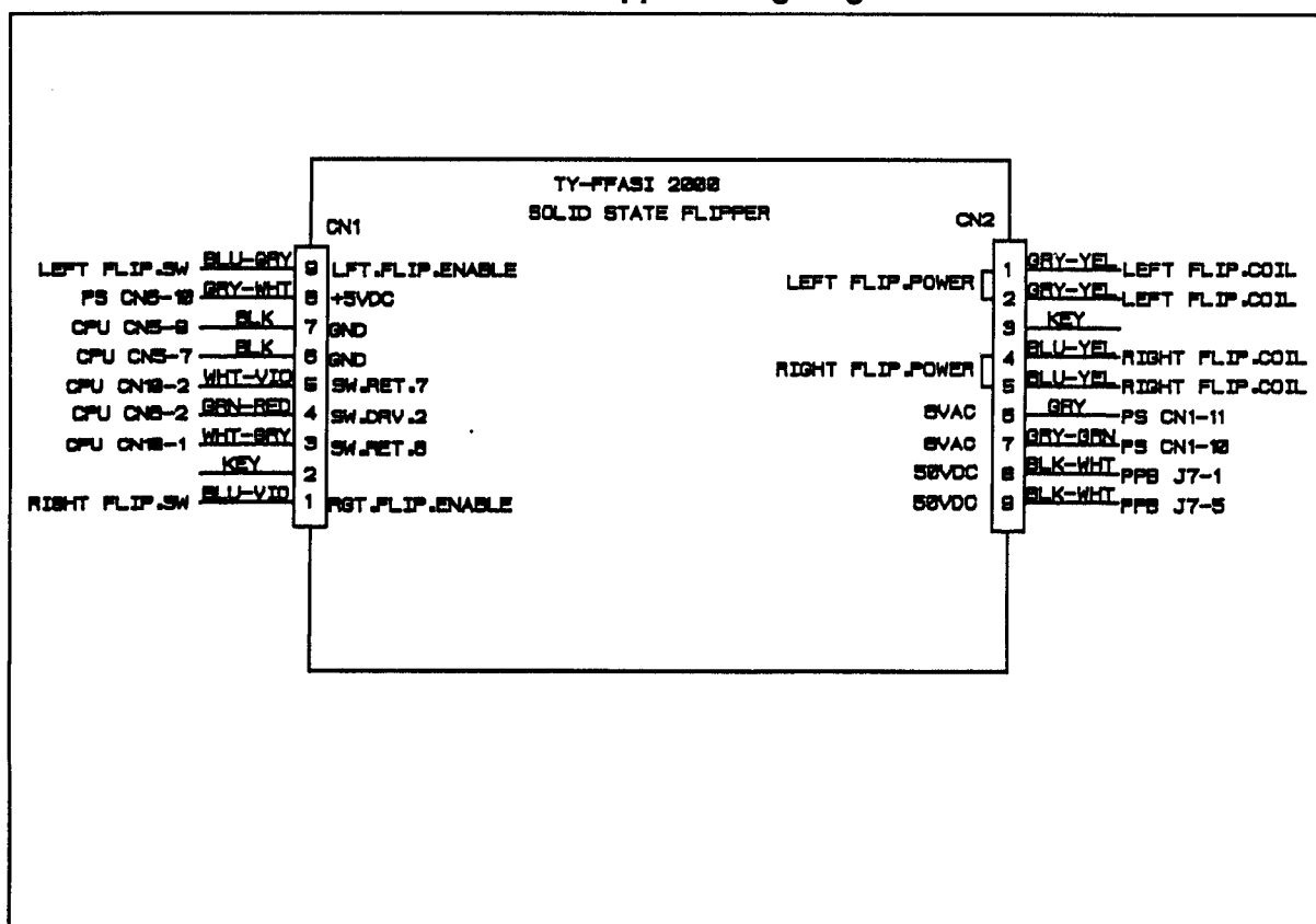
Solid State Flipper Wiring Diagram
