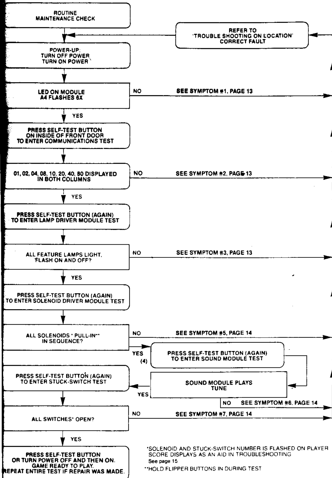
FIGURE IV. SELF-DIAGNOSTIC TEST MPU A4
