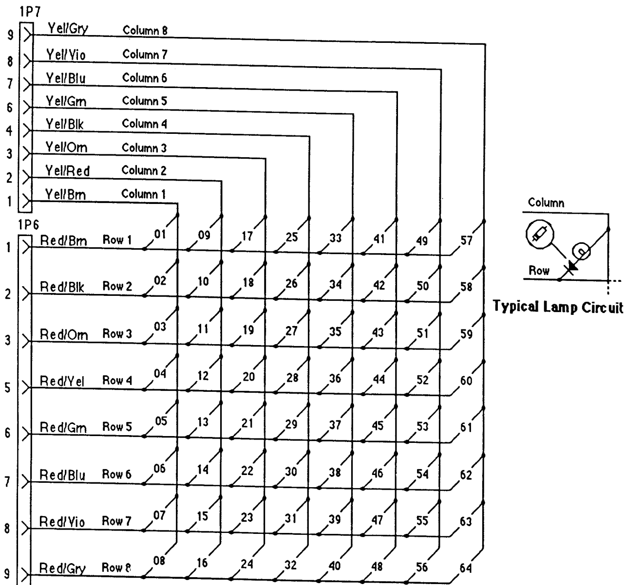
BANZAI RUN Lower Playfield Lamp-Matrix Table
