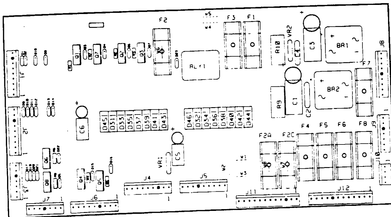
Aux Power Driver Unit Board p/n D-12247-563
