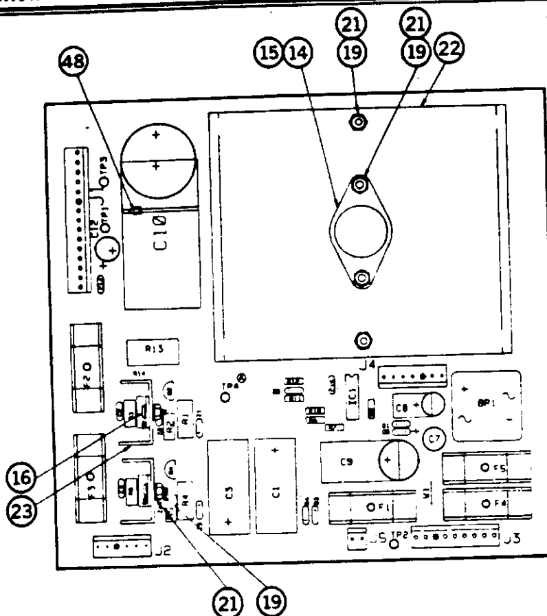
Power Supply p/n D-12246
