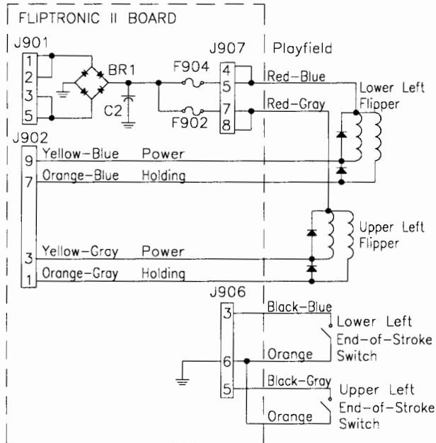
Left Flipper Circuit
