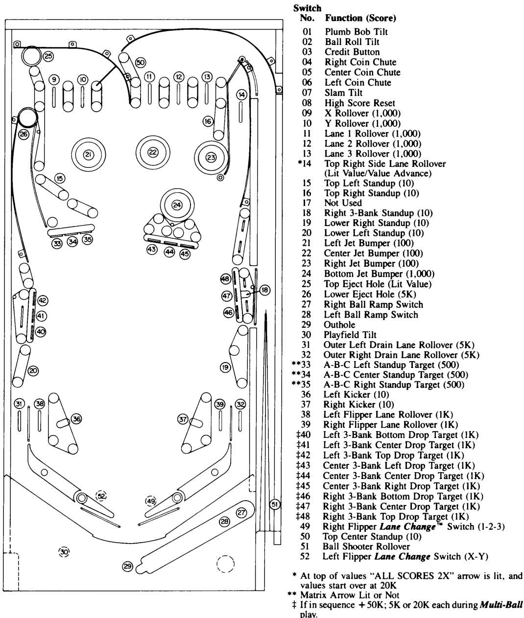
Figure 3. Playfield Switch Locations and Switch Chart
