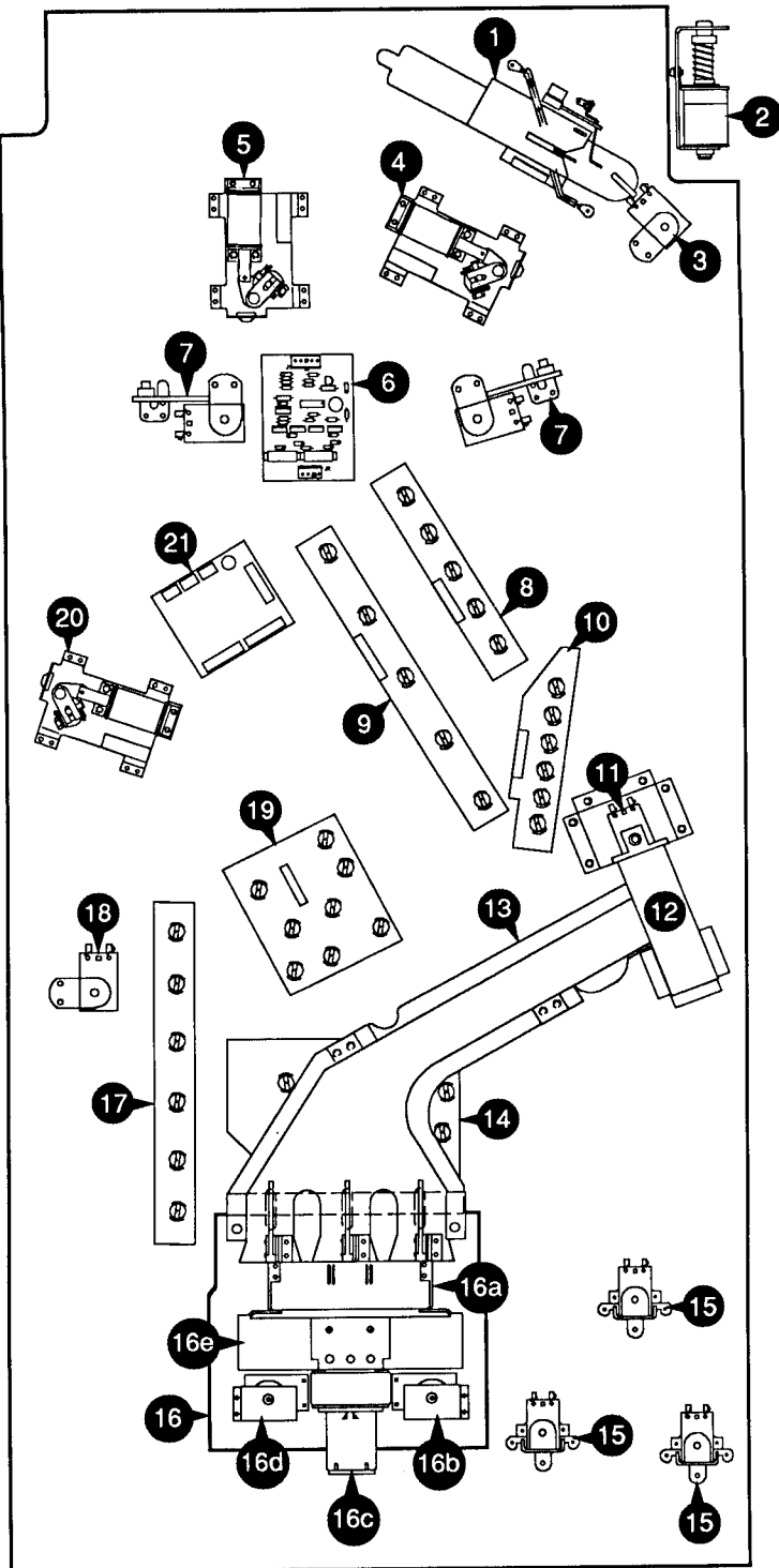
Underside of Playfield, Viewed in Raised Position
