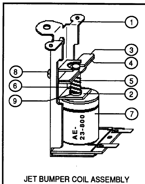
JET BUMPER ASSEMBLY
