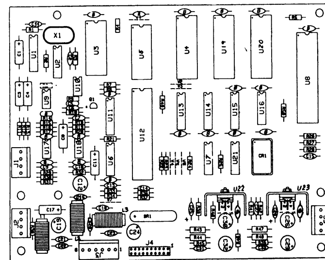
AUDIO BOARD ASSEMBLY p/n D-11581
