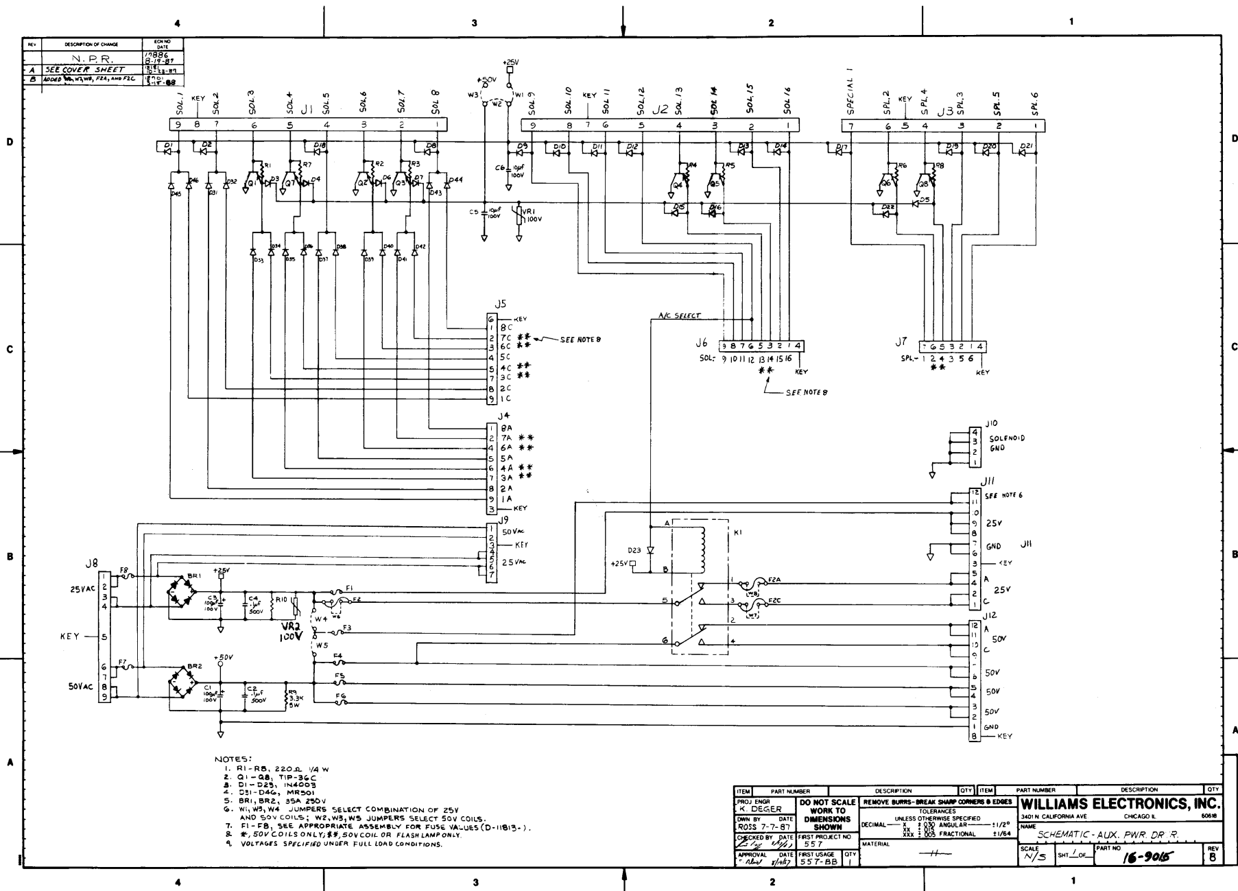
Aux Power Driver Board Schematic
