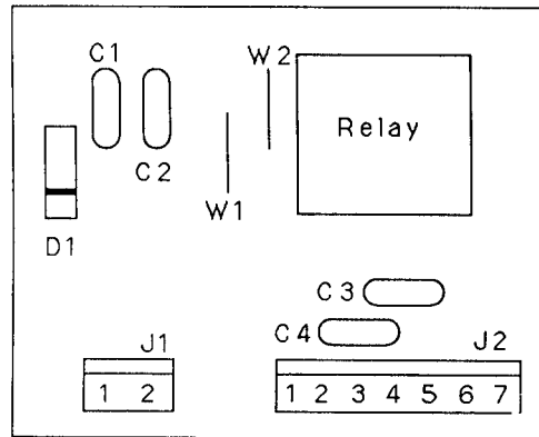
Relay Board
