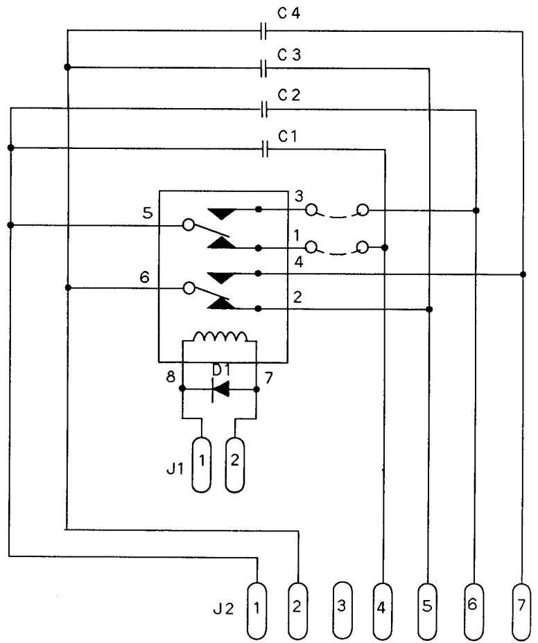
Relay Board Schematic
