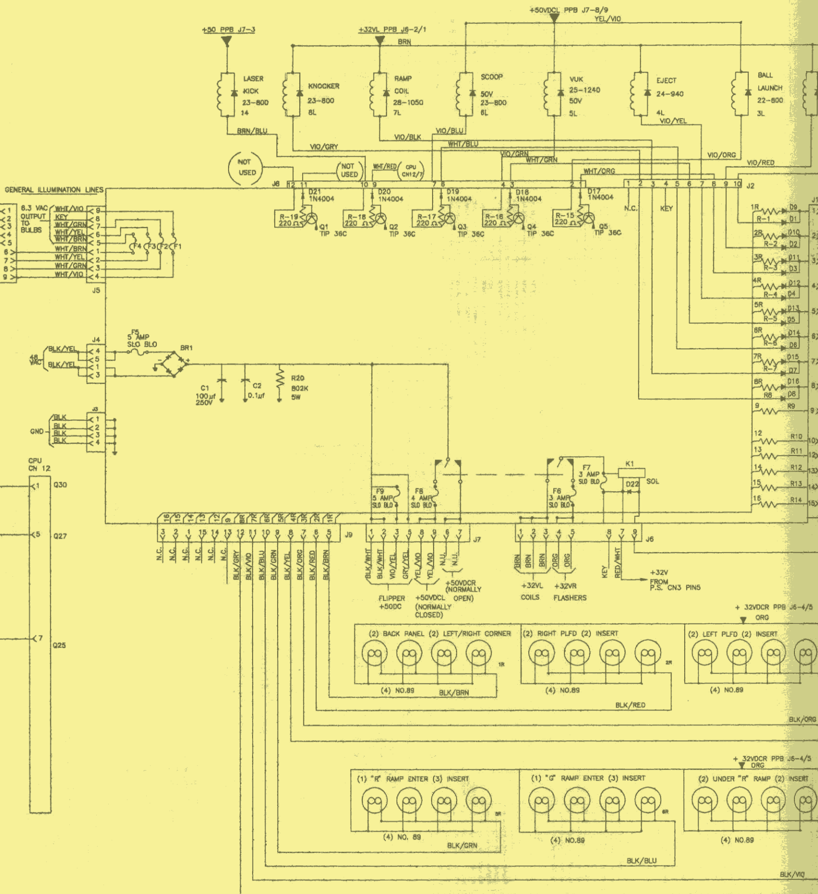
Playfield Coil / Flashlamp Wiring Diagram
