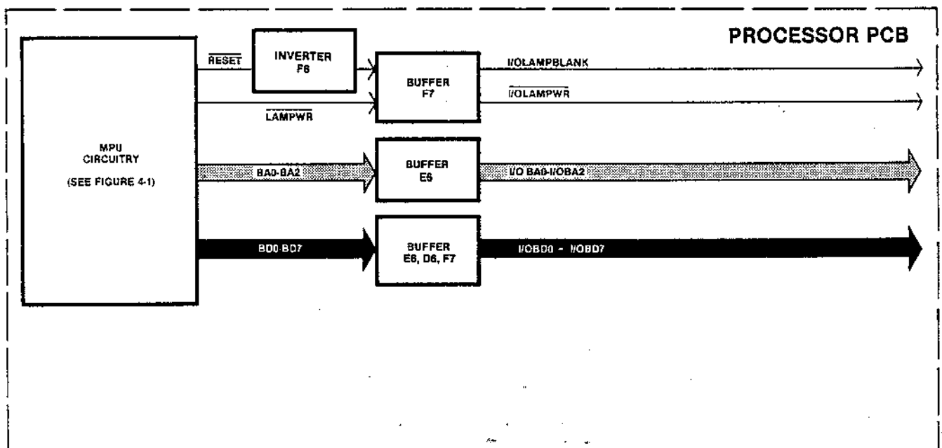
Figure 4-4 Processor PCB
