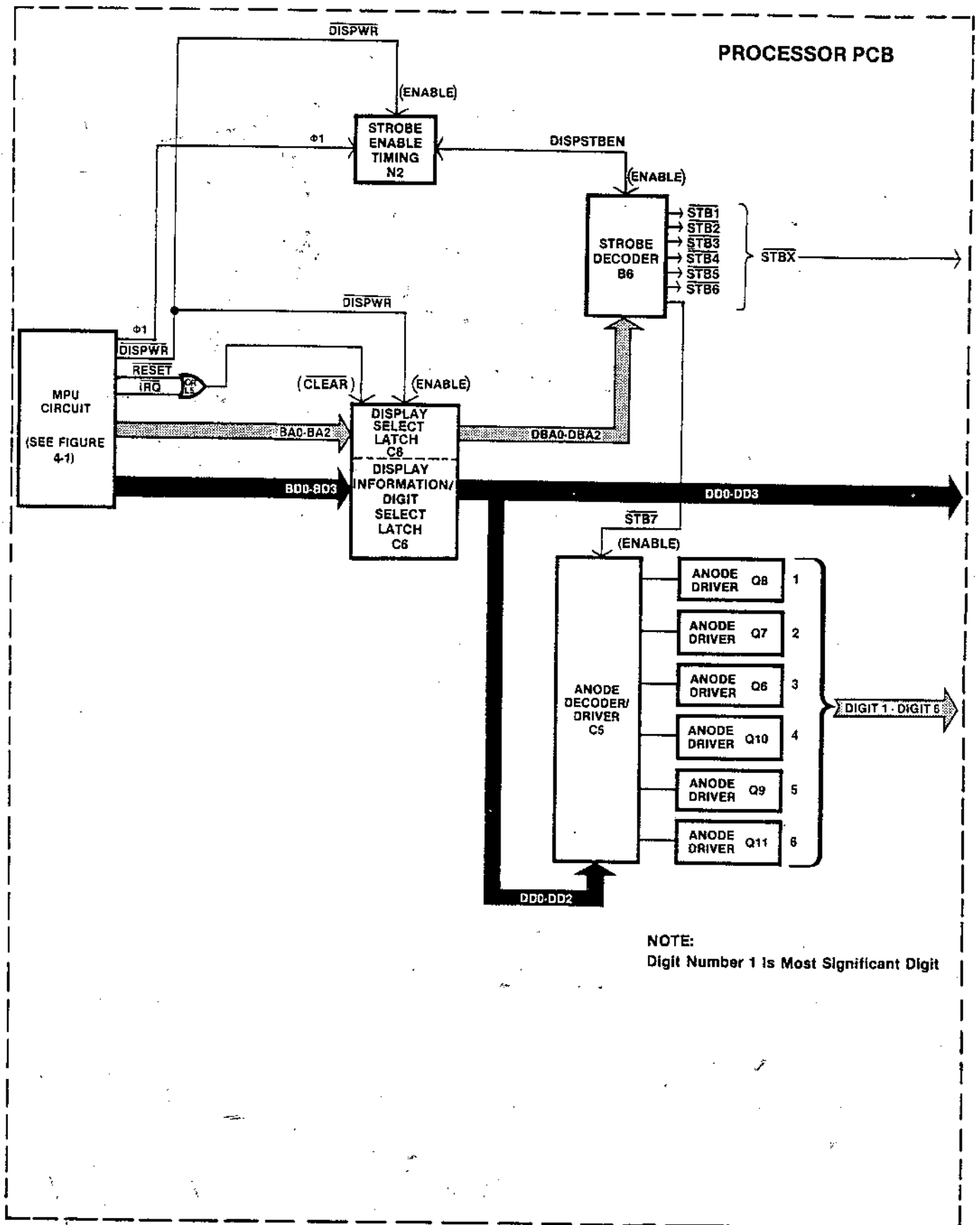
Figure 4-6 Display Circuitry
