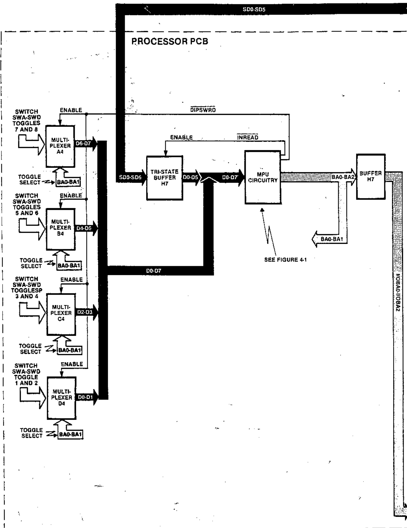
Figure 4-2 Switch Circuitry
