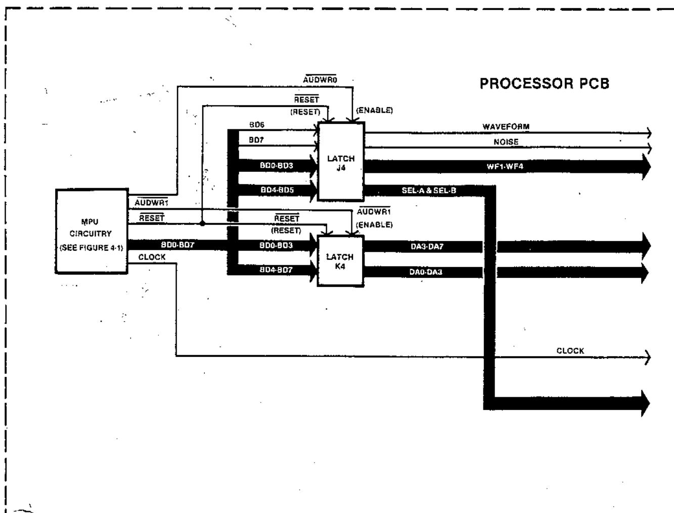
Figure 4-8 Audio Circuitry
