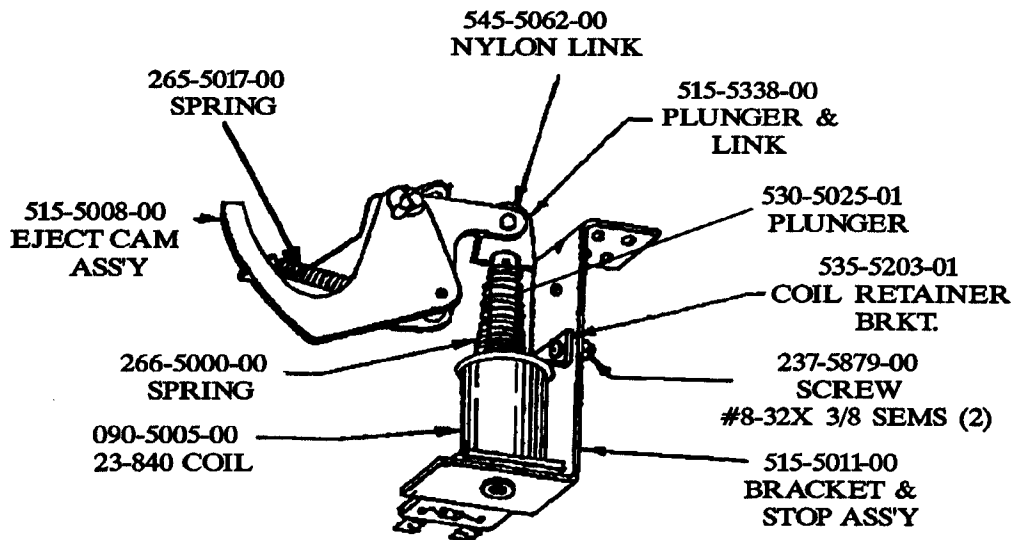
500-5012-01 BALL FEED ASS'Y (TROUGH EJECT)
