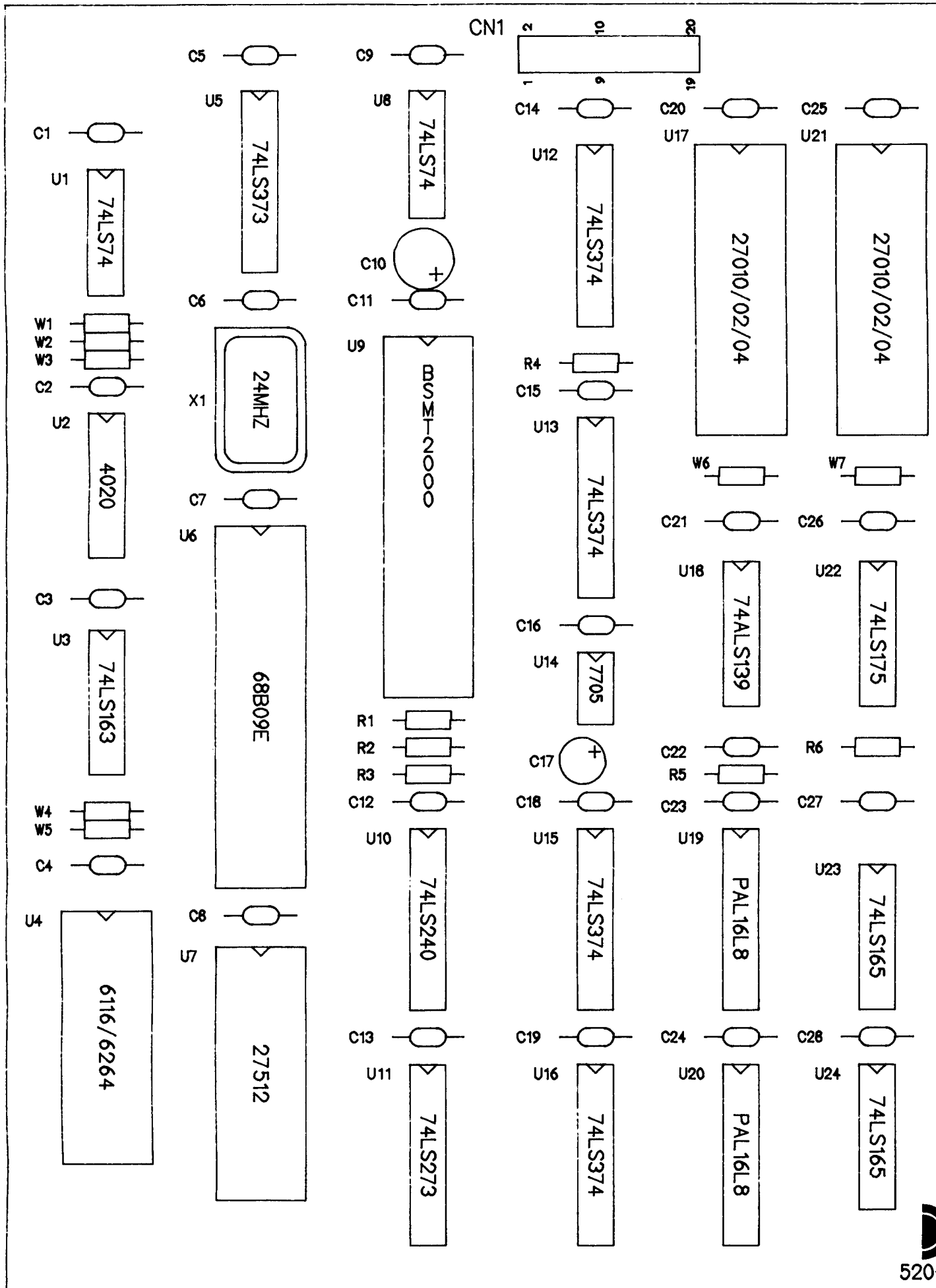
Sound Board Assembly Drawing
