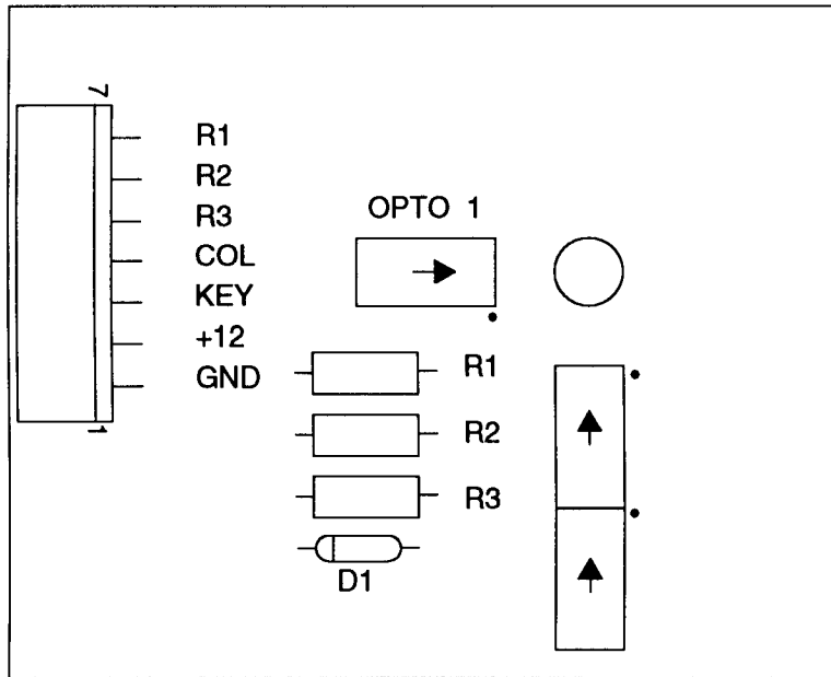
Board Assy.
