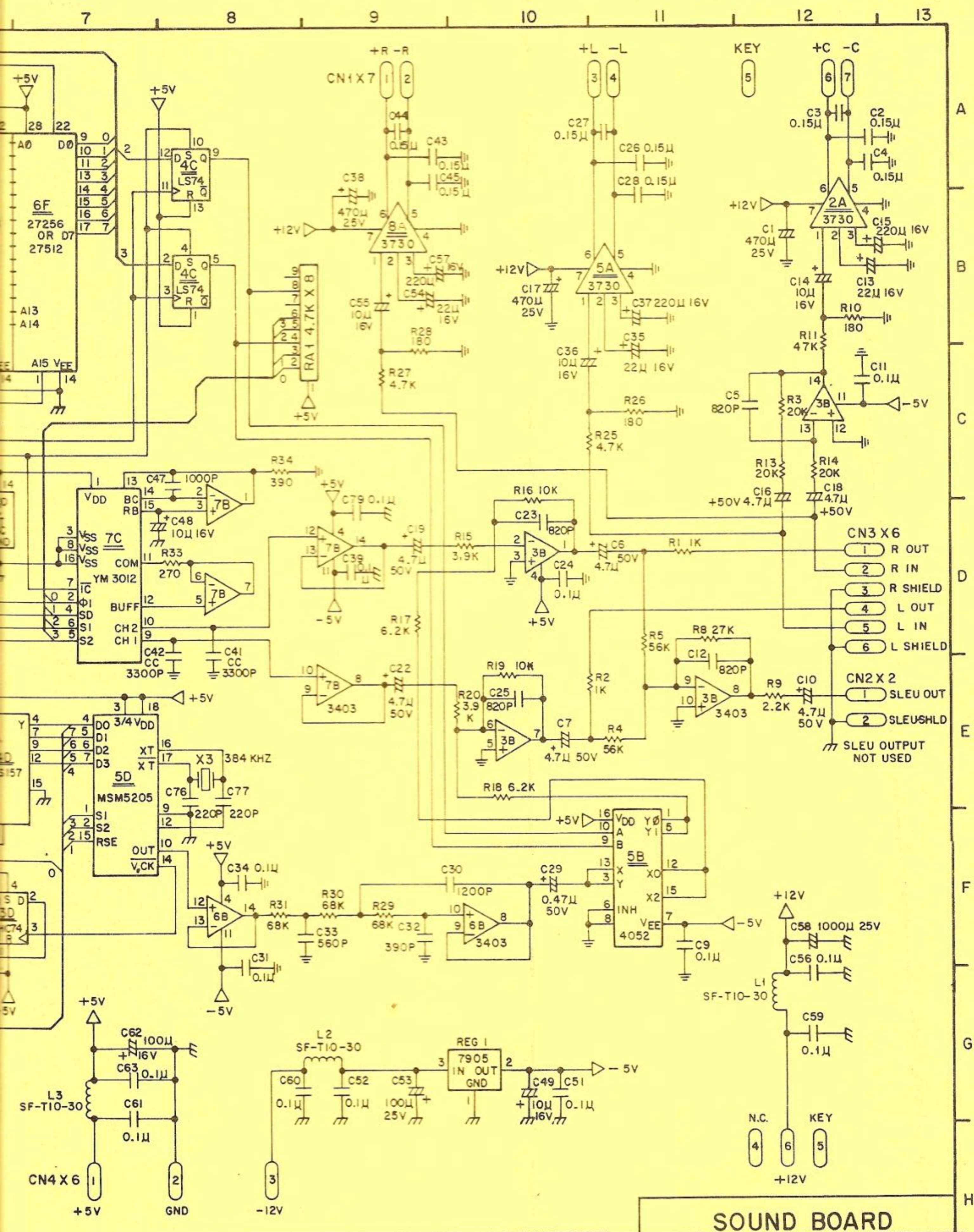
Sound Board Logic Diagram
