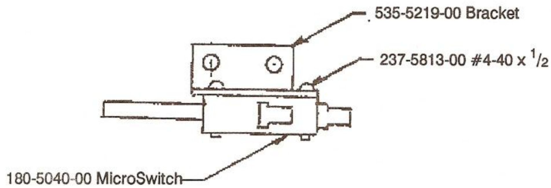
Micro Sw.&Bracket Assembly 515-5084-01 Left (Shown) 515-5084-00 Right
