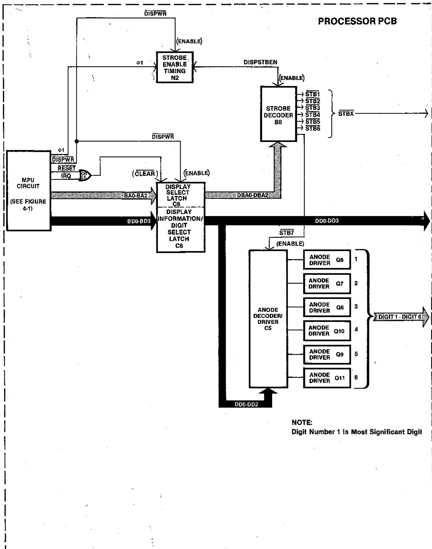
Figure 4-5 Display Circuitry
