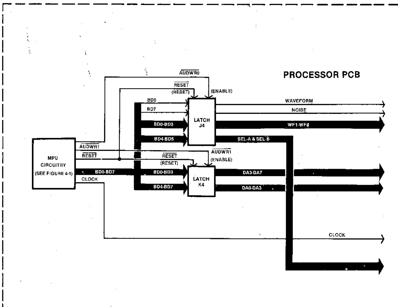
Figure 4-6 Audio Circuitry
