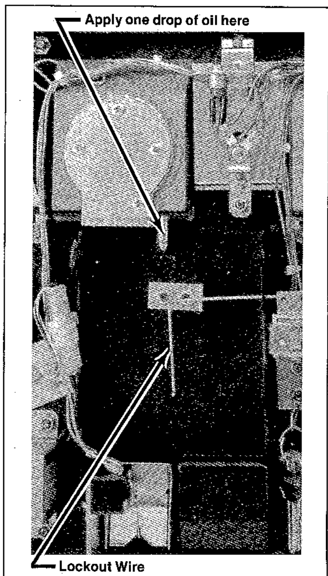
Figure 3-6 Lubrication Point
