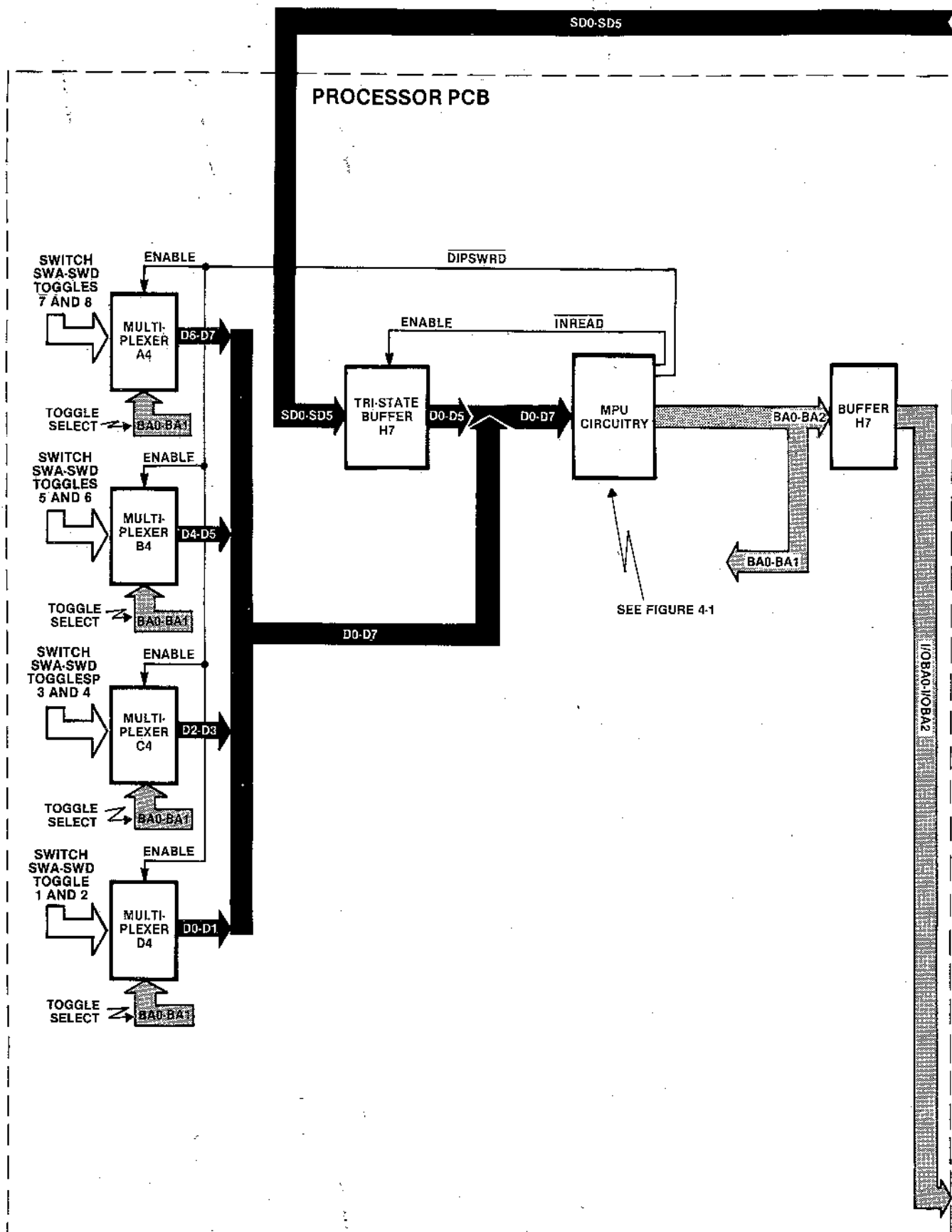
Figure 4-2 Switches Circuitry
